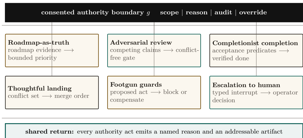
Figure I.5: The authority half (§I.4): six distinct mechanisms by which the consented daemon acts . The common boundary is the recorded grant g : every mechanism takes a legible input, produces a bounded authority result, and returns a named reason with an addressable artifact. Roadmap-as-truth answers what authority is for; adversarial review, completion, landing, footgun guards, and human escalation each constrain a different kind of act. The engineering status of each mechanism is recorded in Appendix I.A.
