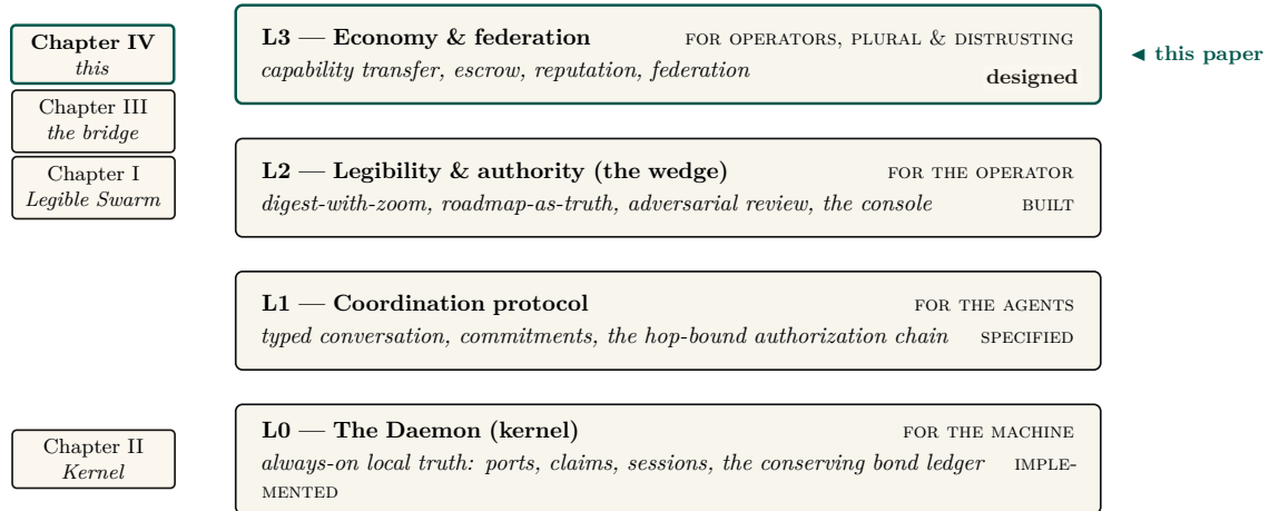
Figure IV.1: This paper is the top rung of a four-layer stack, and it depends on every rung below it. The L0→L3 stack: each rung serves a different whom , and each announces what it assumes from below. Chapters I–III establish legibility, the kernel, and the L3 identity bridge; The Harbor Economy is the top rung — the only layer whose participants are plural and mutually distrusting, and it depends on every rung below it. It consumes the implemented bond ledger from L0, the cryptographic hop-bound authorization chain from L1, and the legible person from Chapter III, and turns them into a market. Chapters V–VII deepen the protocol, incentive, and federation seams; chapter numbers are not layer numbers. The series spine runs up this stack: memory → checkpoint → continuity → a person not a spawn → registered outcomes → reputation → a tradeable asset → the market — the same memory that makes the single-player wedge good is what turns a spawn into a tradeable asset.
