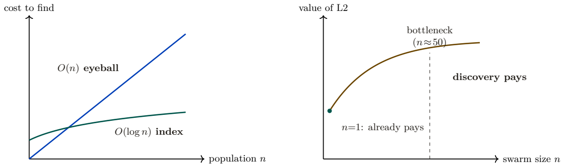
Figure I.9: Read-poverty (§I.6): state piles up faster than it can be read. Left: the cost of finding the right agent/work grows linearly under eyeball search but stays near-flat under an indexed directory — the same trade every database made at the table-scan wall. Right: the value curve of the legibility wedge across swarm size. It is valuable already at n=1 (briefing, attestation, footgun guard, honest completion) and grows into the read-poverty regime; discovery ranking earns its keep around the n \approx 50 bottleneck. The wedge must work at n=1 and grow gracefully.
