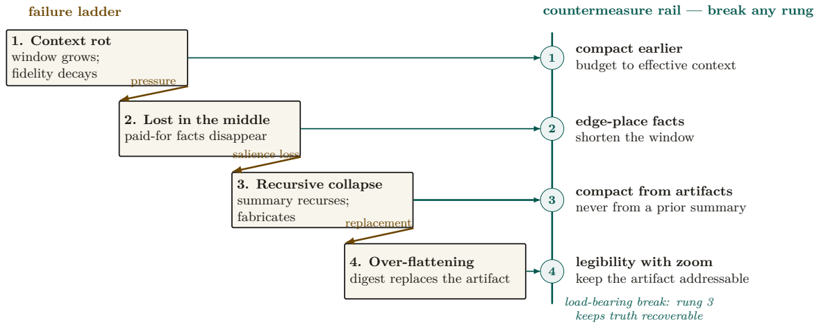
Figure I.13: The context-degradation cascade (§I.8.4): rot makes you compact, naive compaction loses the middle, recursion fabricates, and the operator-facing digest over-flattens what remains. The amber ladder encodes the causal order; the parallel teal rail places one countermeasure at each rung, so breaking any rung stops the cascade. The load-bearing intervention is compact-from-artifacts (rung 3): durable, addressable claims, notes, and episodes make it possible to reconstruct a digest from evidence rather than from a previous summary. When compaction fails, the bill and the truth degrade together.
