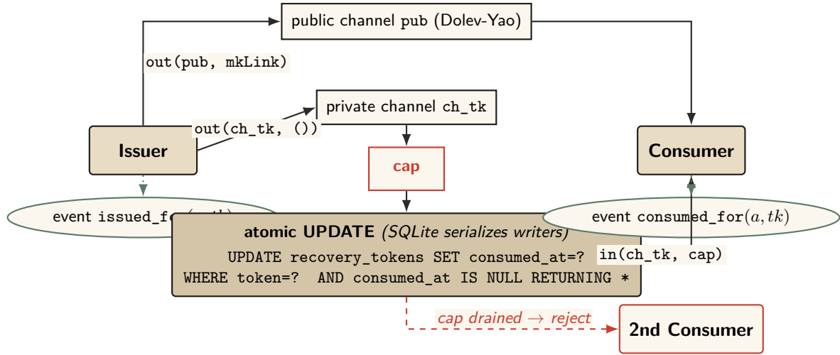
Figure 6: Magic-link single-use atomicity. The SQL UPDATE ...WHERE consumed_at IS NULL RETURNING is the runtime analogue of the ProVerif private-channel cap : SQLite serializes concurrent writers, so the first caller drains the cap and the second consumer’s transaction returns zero rows. Verified properties: injective single-use ( \text{inj-event}(\text{consumed\_for}) \Rightarrow \text{inj-event}(\text{issued\_for}) ) and binding.
