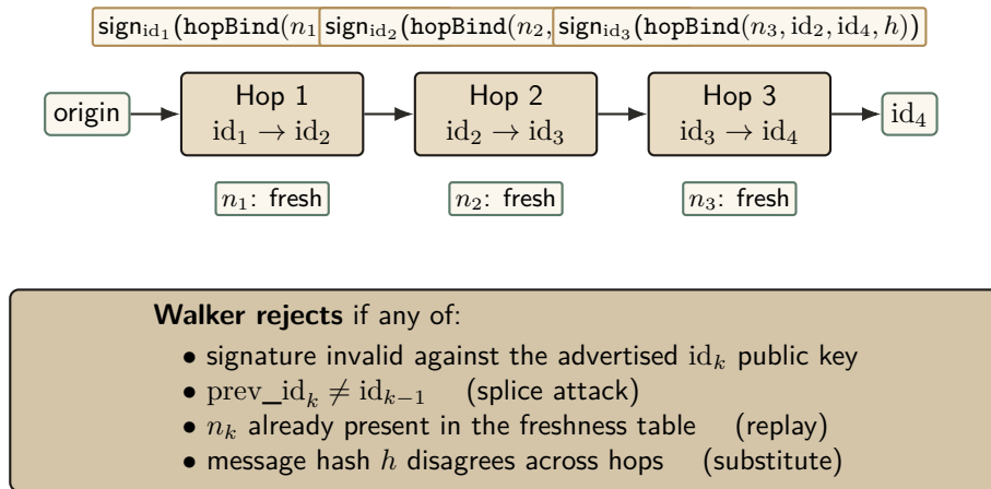
Figure 7: Multi-hop delegation walker. Each hop k signs a binding tuple (n_k, id_{k-1}, id_k, h) under Ed25519, where h is the message hash that must remain constant across the chain. The walker verifies depth- N chains with a nonce-freshness table and rejects splices, replays, hop-swaps, and substitution.
