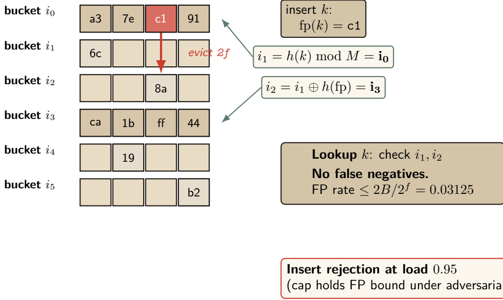
Figure 8: Cuckoo filter (Fan et al. [23]). 8-bit fingerprints, 4 entries per bucket, partial-key cuckoo hashing. Insert lands at either of two candidate buckets i_1, i_2 = i_1 \oplus h(fp) ; on full, evict and re-insert at the kicked fingerprint’s alternate. The runtime caps load factor at 0.95 to keep occupancy inside the regime where the false-positive bound holds.
