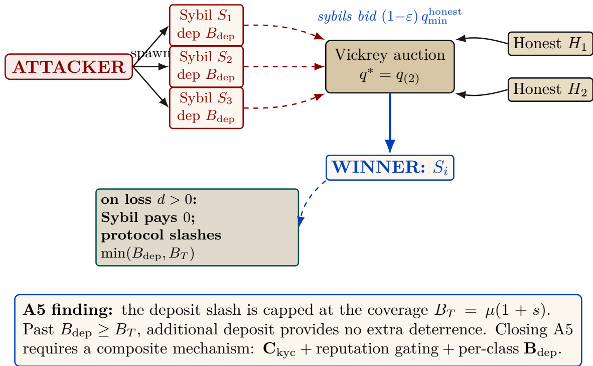
Figure 6: Sybil attack flow. The attacker spawns K Sybil identities, each posting deposit B_{\text{dep}} , then undercuts honest bids by \varepsilon and defaults on loss. The protocol confiscates the Sybil’s deposit on default, but the slash amount is capped at the coverage B_T — so beyond B_{\text{dep}} \geq B_T additional deposit provides no extra deterrence. Empirically demonstrated in Figure 7.
