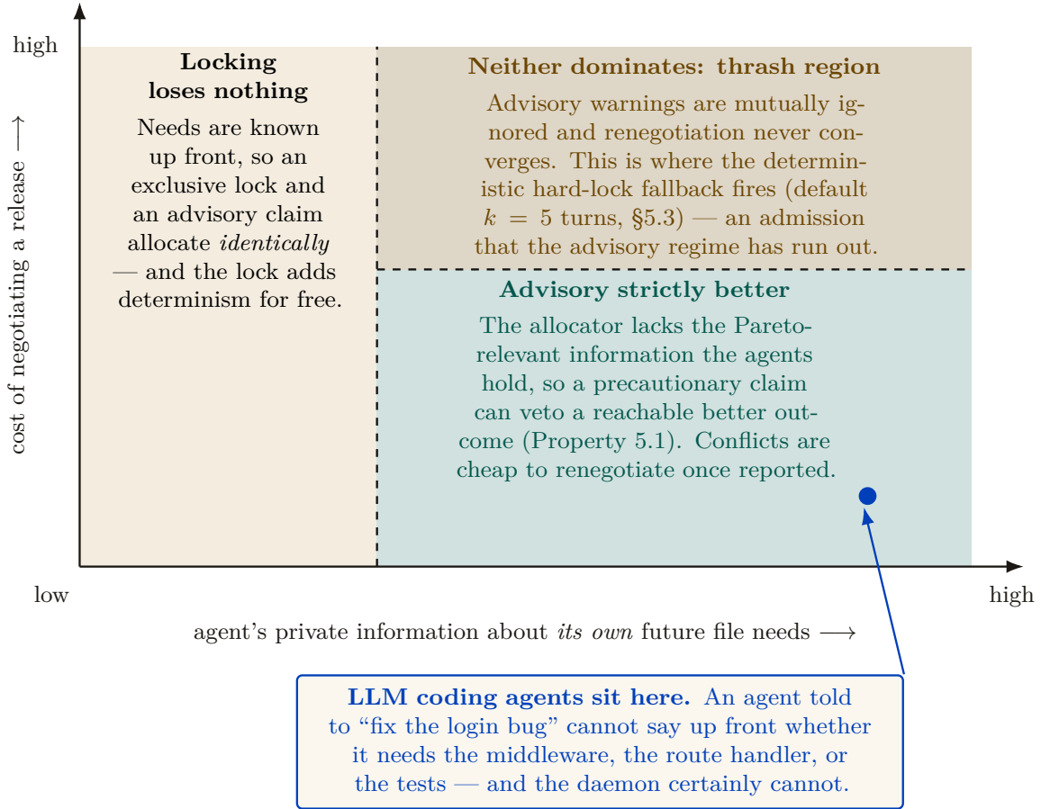
Figure 2: Advisory claims do not beat enforced locks everywhere — they beat them only to the right of the dashed vertical, where agents hold private information the allocator cannot have. To its left, locking costs nothing and buys determinism, so Sen’s warning does not apply and this paper’s design choice would be wrong. Above the dashed horizontal, neither regime works and the hard-lock fallback of §5.3 takes over. The marked point is where LLM coding agents actually sit, which is the entire argument for the advisory default of §5.2.
