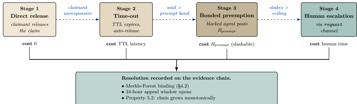
Figure 3: Governance and appeals: four-stage escalation path. The daemon resolves most disputes at stage 1 or 2 (zero or near-zero cost). Bonded preemption (stage 3) prices the blocked agent’s claim that the holder is wrong; if the preemption is wrong, the bond is slashed under settlement. Human escalation (stage 4) is reserved for the cases the daemon cannot mechanically decide. Every resolution is appended to the evidence chain with the same Merkle-Forest binding as any agent action, so all four stages remain auditable.
