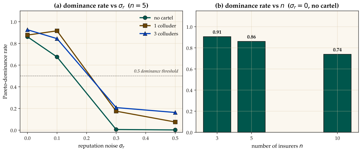
Figure VI.4: Monte Carlo comparison of competitive auction and the specified static-escrow baseline. Left: fraction of trials satisfying the code’s Pareto criterion versus reputation noise \sigma_r at n = 5 , split by cartel size. Right: the same criterion versus insurer count at \sigma_r = 0 with no cartel. Error bars and seeds are recorded in the accompanying artifact; the curves are not analytical welfare bounds.
