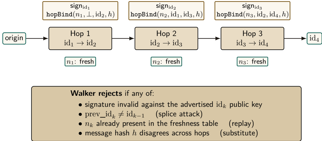
Figure V.4: Multi-hop delegation walker. Each hop k signs the binding tuple (n_k, id_{k-1}, id_k, h) under Ed25519, where h is the message hash that must remain constant across the chain. The walker verifies depth- N chains with a nonce-freshness table and rejects splices, replays, hop-swaps, and substitution. Runtime: lib/delegation-chain.ts ; ProVerif conformance test passes 17 / 17.
