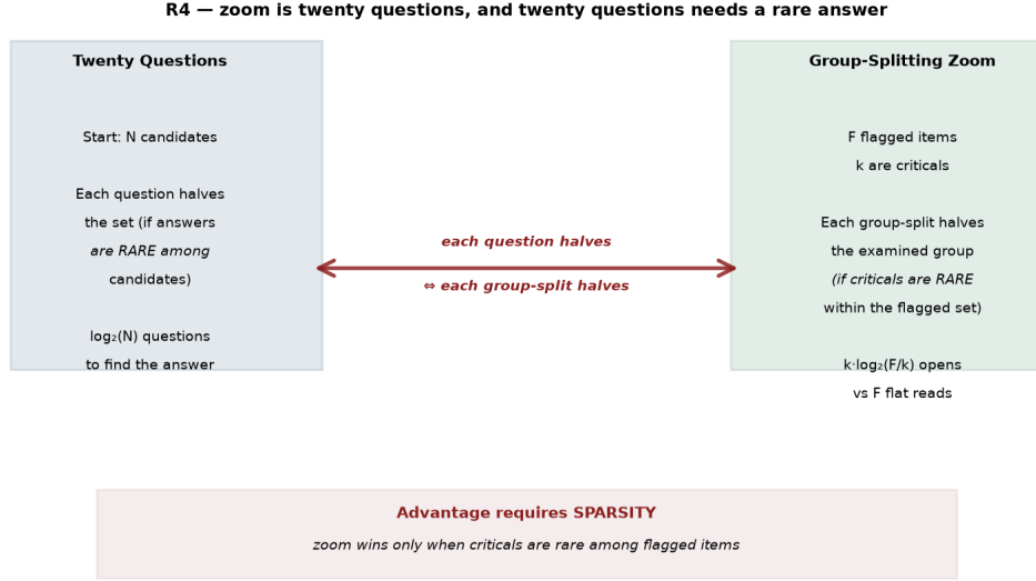
Figure 5: The relation-map for zoom: twenty questions (base) against group-split inspection of the flagged set (target). The correspondence that does the work is “one question halves the candidate set when answers are rare ”; the misread it invites — that \log_2 F questions suffice — is exactly what Theorem 4’s 2k \lceil \log_2(F/k) \rceil + 4k accounting corrects for k > 1 .
