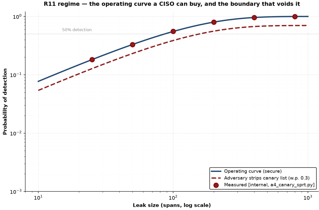
Figure 4: Regime diagram for Pillar IV: the operating curve a CISO can buy, and the boundary that voids it. Left: \Pr(\text{detect}) against leak size m at density 1%, \beta = 0.2 — exact, approximate, and simulated agree [internal, a4_canary_sprt.py ]. The guarantee’s load-bearing regime is secret, uniform planting: an adversary who obtains the canary list with probability 0.3 and strips all of them drops measured power from 0.9997 to 0.698 at k=5 [internal].
