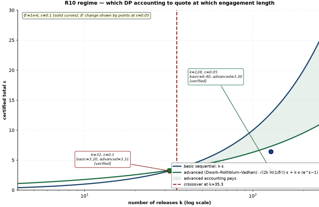
Figure 3: Regime diagram for Pillar III: which DP accounting to quote at which engagement length ( \delta' = 10^{-6} ). Below the crossover in k the sequential bound k\varepsilon is exact, \delta -free, and smaller; past it, advanced composition’s \sqrt{k} scaling wins. The session’s two measured points ( k=32, \varepsilon=0.1 and k=128, \varepsilon=0.05 ) are marked [verified; regenerated by a3_epsilon_ledger.py ].
