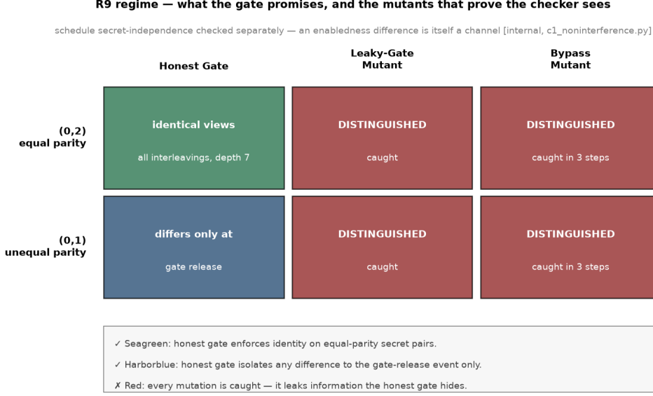
Figure 2: Regime diagram for Pillar I: what the gate promises, and the mutants that prove the checker sees. The property holds on the shaded region (equal declassified value, any interleaving); the two mutation witnesses (leaky gate; gate bypass) sit provably outside it, each with a concrete trace [internal, c1_noninterference.py ].
