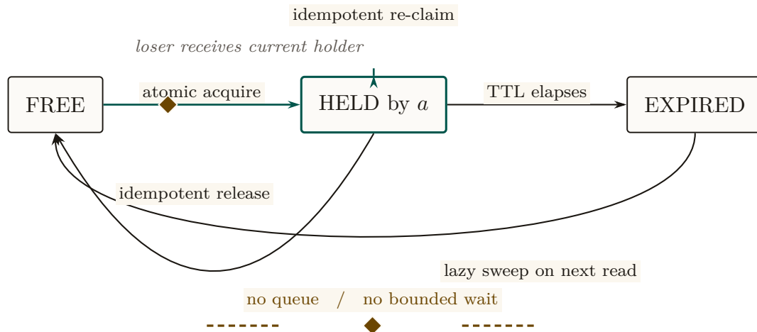
Figure 5: The guarded claim lifecycle. Acquire is one atomic uniqueness decision; re-claim and release are idempotent; expiry is removed lazily on the next read. The interrupted amber rail is intentional negative space: the kernel has no queued state and therefore no fairness or bounded-wait guarantee. A reactive ticket mechanism may later occupy that gap for cooperatively released claims, but lazy expiry would still bypass it, so starvation remains an open problem.
