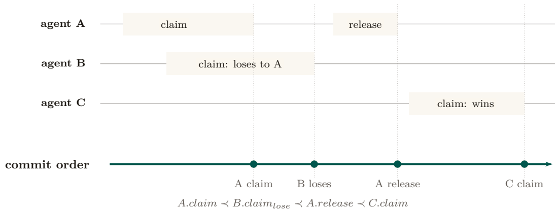
Figure 13: A real-time history and its extracted linearization. Operations may overlap in caller time, but each receives one commit point on the single writer’s rail. Those points explain the observable result without a prose table: A wins, B overlaps but loses to the recorded holder, A releases, and only then can C win. The claim is conditional on one writer, no uncommitted reads, and replies after commit; a bypass would destroy the correspondence.
