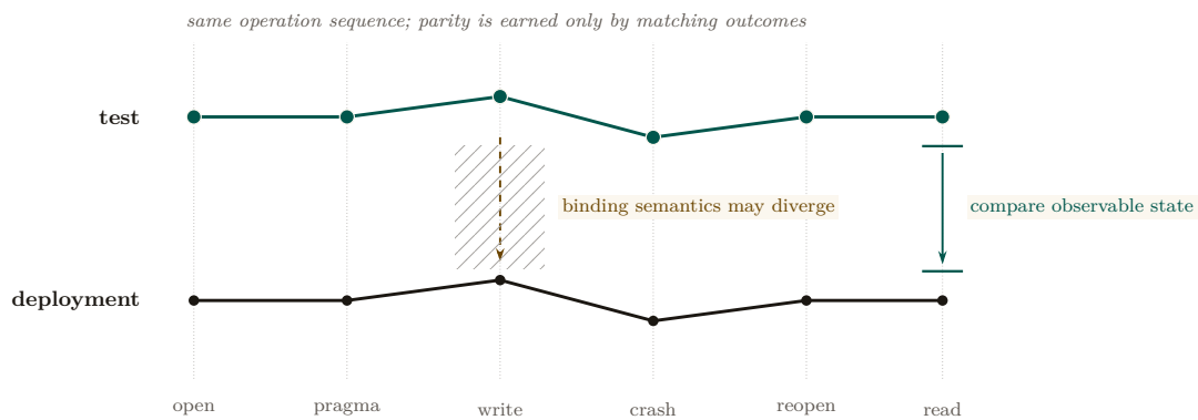
Figure 14: Runtime parity as a trajectory comparison. The same operation sequence is applied to the test binding and to the compiled deployment daemon; the harness must compare observable state after reopen, not merely confirm that both programs build. The hatched gap is the unproved surface where pragma, locking, or checkpoint semantics can diverge. A shim aligns interfaces, but only booting the deployment runtime and differential testing can collapse that gap into a verified invariant.
