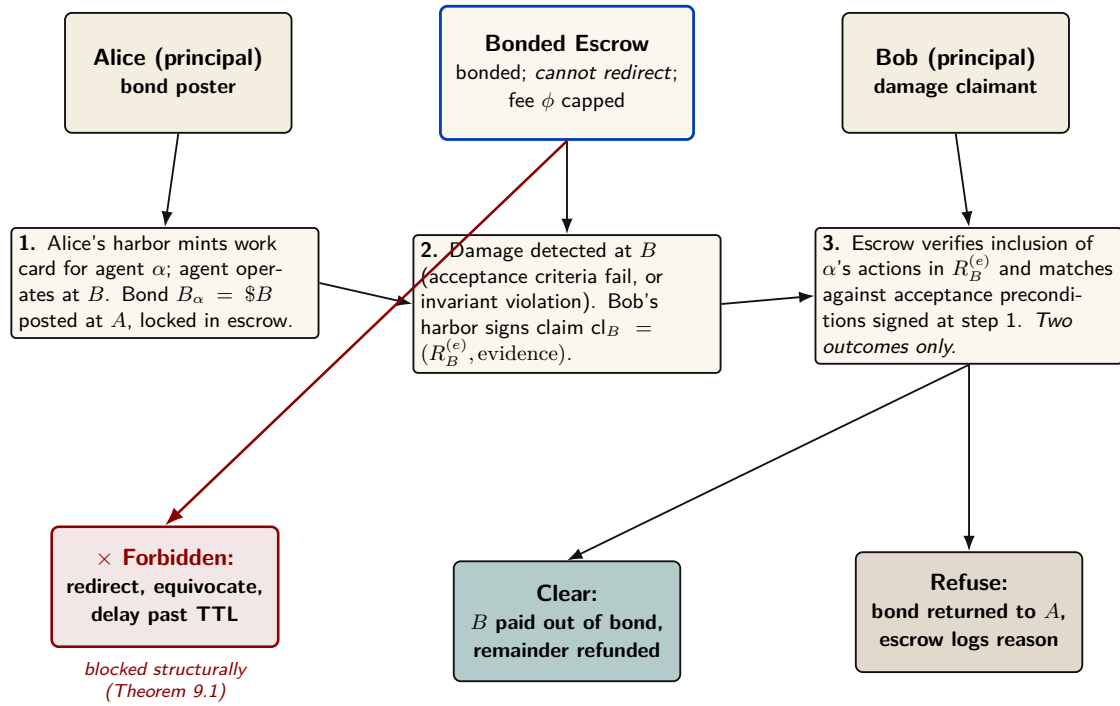
Figure 9: Cross-harbor settlement protocol. The escrow is a third party in the sense that neither A nor B alone can compel an outcome, but it is not a trusted third party in the operational sense: the protocol restricts its decision space to two outcomes (clear or refuse) and prices its maximum extractable fee \phi up front. Redirecting funds, equivocating about a clearing decision, or delaying past TTL are structurally forbidden by the property checks in Theorem 9.1. The escrow is a bounded third party — the bond it holds plus the cap on \phi make its misbehavior bounded-loss rather than catastrophic.
