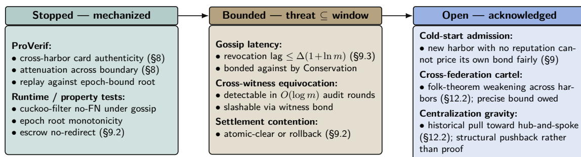
Figure 11: Threat-band layout for the Federated Harbor. The Anchor paper’s defense-in-depth structure carries over: every claim either has a mechanization artifact (teal), a named bound that the bond can price against (amber), or an explicit acknowledgement of the open frontier (cobalt). The paper is disciplined about which band each claim lives in — see Appendix A for the artifact registry. Reading left to right runs deeper into threat space and out of formal reach; bands shift left over time as future work mechanizes what is presently bounded.
