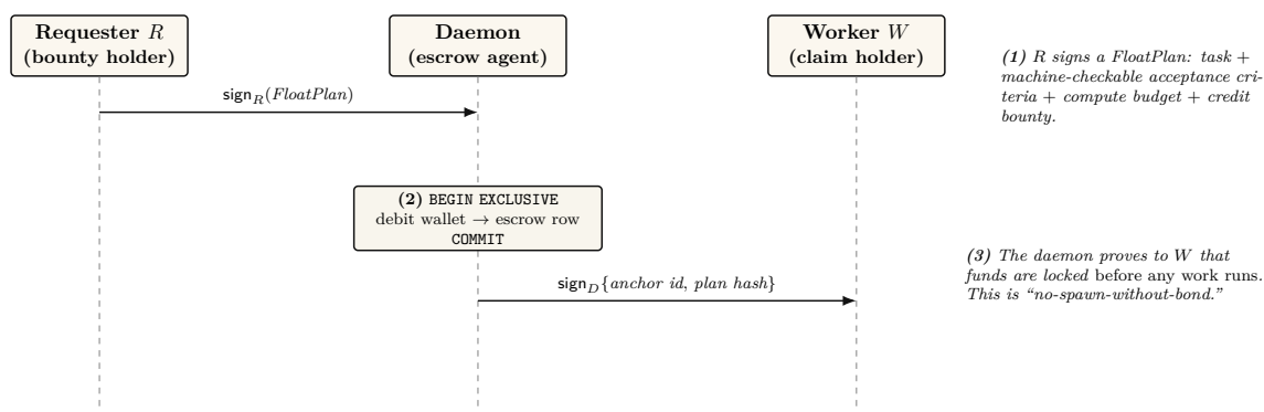
Figure 4: The float-plan escrow ceremony — the atom every side of the market settles on. A three-step signed handshake over a standard digital-signature scheme: the requester signs a FloatPlan (task, machine-checkable acceptance criteria, budget, bounty); the daemon debits and escrows the value inside one serialized database transaction; the daemon then signs \{\text{anchor id}, \text{plan hash}\} , proving to the worker that funds are pinned before any work begins. The conservation invariant (wallet + escrow + commons = supply, verified over 10k random operation traces by a property test) holds at every step and is the implemented floor the whole economy stands on — the one claim this paper can make at the highest maturity.
