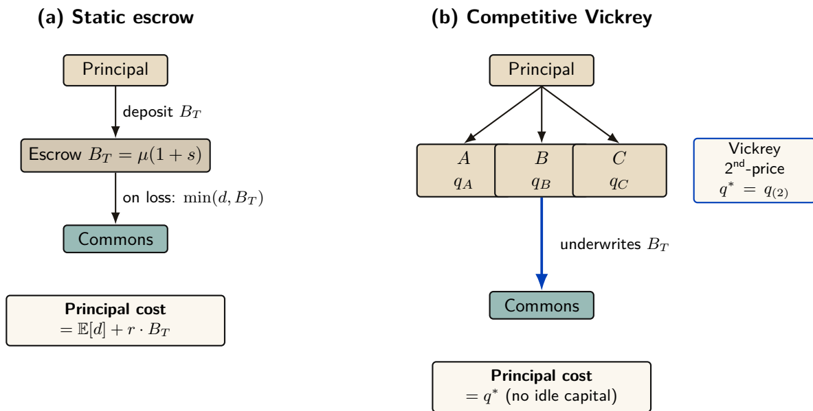
Figure 13: Static escrow vs. competitive Vickrey auction. Both regimes underwrite the same coverage B_T = \mu(1 + s) ; only the financing mechanism differs. In (a) the principal ties up B_T for the coverage period, paying an opportunity cost r \cdot B_T . In (b) insurers compete; the principal pays only the second-lowest bid q^* . The competitive regime Pareto-dominates the static one under the welfare assumptions of §12.1 below.
