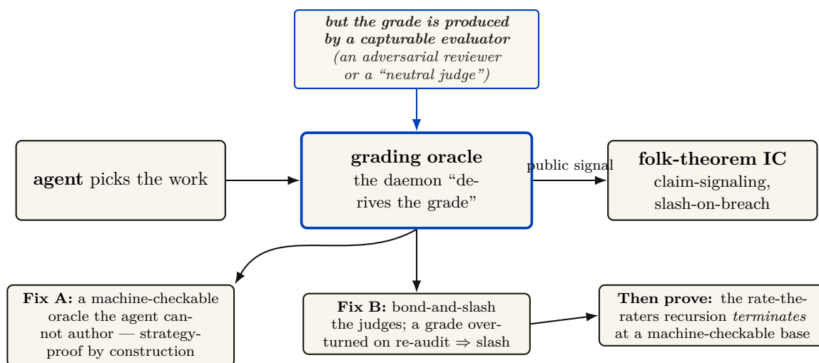
Figure 12: The grading-oracle incentive-compatibility problem — the hole under the core theorem. Every folk-theorem claim in the layer bottoms out in “the agent picks the work, the daemon derives the grade.” But a folk theorem is only as good as the public signal it conditions on (Green–Porter 1984; Abreu–Pearce–Stacchetti 1990 require the signal distribution to be common knowledge and exogenous ). The grade is produced by a capturable evaluator, so the signal is endogenous and the folk theorem does not apply as stated. We resolve it two ways: ground settlement in machine-checkable oracles the agent cannot author (Fix A, strategy-proof by construction), and bond-and-slash the human/LLM judges where machine-checking is impossible (Fix B), then require the rate-the-raters recursion to terminate at a machine-checkable base.
