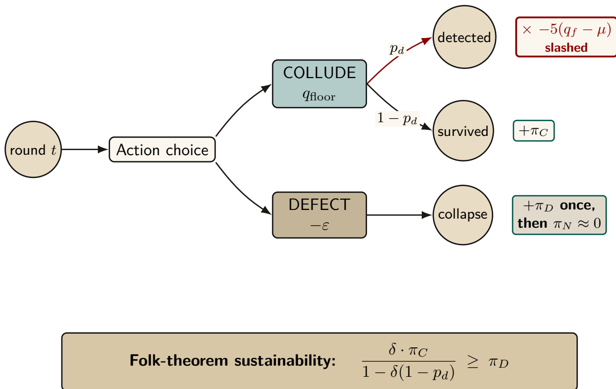
Figure 14: Cartel repeated-game node under the grim-trigger strategy. Each round a colluding member chooses between maintaining the floor q_{\text{floor}} or undercutting it by \varepsilon . Detection (probability p_d ) lands on the red \times path: the colluder is slashed -5(q_f - \mu) . One-shot defection takes the \pi_D gain once, then collapses the future \pi_C stream to \pi_N \approx 0 . The cartel is self-sustaining exactly when the inequality at the bottom holds; raising p_d (sampled adversarial re-audit) or capping \pi_C (diminishing-returns concavity on pairwise outcomes) pushes the critical discount factor past 1 and breaks it.
