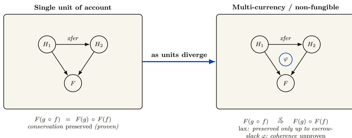
Figure 6: Conservation as a (lax) functor. Within a single unit of account the map F : \mathbf{Harbor} \rightarrow \mathbf{Federation} is a conservative functor : it preserves the composition of settlement morphisms, so the per-harbor invariant wallet + escrow + commons = supply lifts exactly to the federation (proven). The moment harbors price bonds in heterogeneous units, F is at most a lax functor — conservation is preserved only up to the bounded-escrow slack \varphi , and the coherence conditions are unproven. The headline “conservation composes upward” is licensed only with this scope rider. The three cross-harbor open problems (settlement, equivocation, unit-of-account) are one sheaf-gluing obstruction in disguise; the double-spend race is literally the non-vanishing of the first cohomology H^1 of the gluing.
