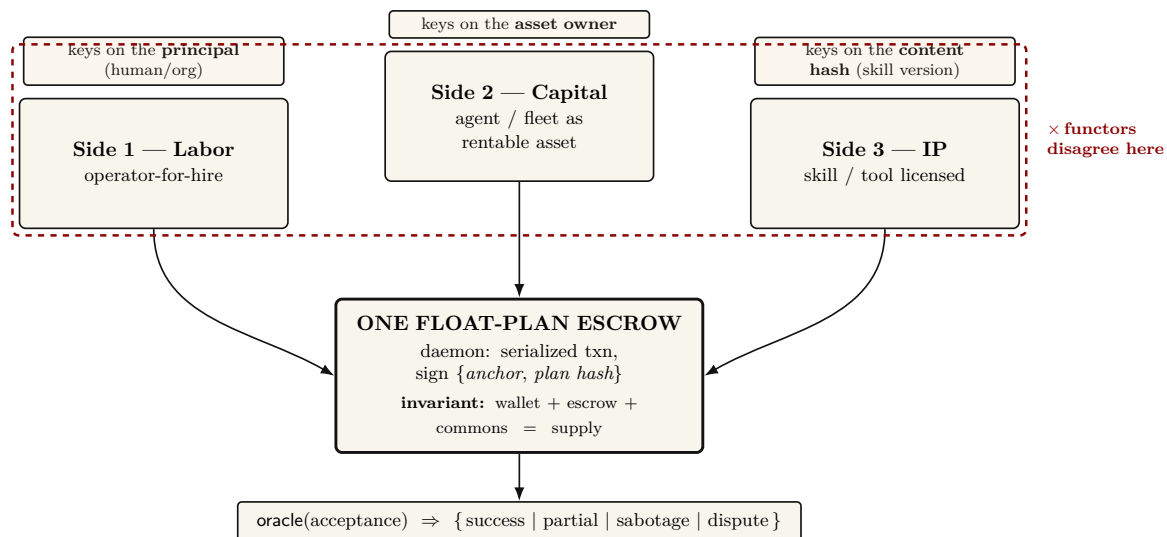
Figure 3: The three-sided market. Labor, capital (rented agents), and IP (licensed skills) are three distinct incentive constraints — not three UI tabs — that all settle on a single float-plan escrow, so conservation holds globally without a second ledger. This is the categorical heart of the design: the three sides are isomorphic at the conservation object (the escrow) and non-isomorphic at the identity object — each side keys reputation on a different entity, so the three partial functors disagree there (the dashed-red band, marked ×). Calling it “one structure, three decorations” without that qualifier is a decorative-analogy failure. The rider is mandatory: the market is three-sided by design and two-sided in shipped reality, because sides 2 and 3 presuppose a non-forgeable, durable identity (§6). The economics per side: labor’s margin is bounty — slashed sub-bonds — fee; capital’s renter holds the runtime jail while the owner bears reputation; IP is metered with clawback, paid only on green settlement. The escrow and its conservation invariant are built and property-tested.
