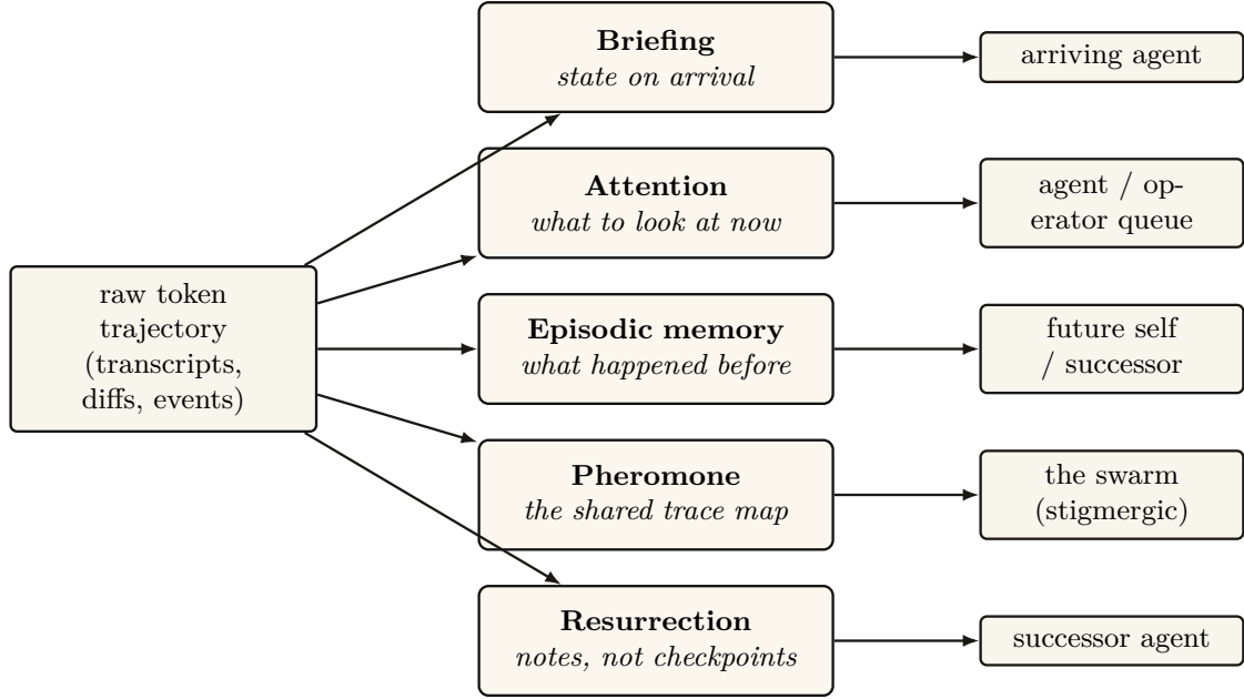
Figure 9: Five read-surfaces, each a token-compaction of the raw trajectory produced for a specific reader (§8.2): briefing is external note-taking, attention is precision compaction, episodic memory is recall-then-precision, pheromone is time-decay (forgetting), resurrection is a handoff summary. Viewed correctly, the swarm’s coordination layer is a distributed compaction engine — and because each surface is a compaction, each is governed by the same cost-and-legibility economics, the same recency-decay (Prop. 7.1), and the same one law (Def. 3.1).
