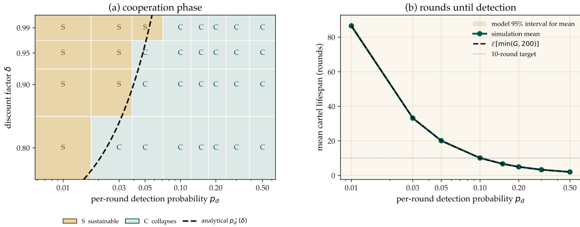
Figure VI.9: Cartel sustainability collapses sharply once per-round detection crosses a narrow threshold: at \delta = 0.95 the closed-form p_d^* \approx 0.0478 and the simulated grid first flips to “collapses” at p_d = 0.05 , a near-exact match. Left: the tested (p_d, \delta) grid under the supplied grim-trigger payoff model; amber cells marked S are sustainable, teal cells marked C collapse, and the dashed curve is the analytical boundary p_d^*(\delta) . Right: simulated mean rounds to first detection, the truncated-geometric expectation, and its model-derived 95% interval for the sample mean. Neither value transfers to a different payoff, event timing, or monitoring model without re-derivation.
