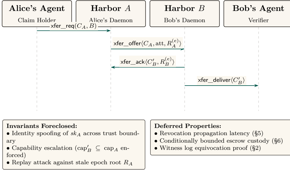
Figure 3: The four-message cross-harbor capability transfer ceremony. The critical property is that no message after (3) needs to reach back to Harbor A in the hot path: C'_B is verifiable under sk_B alone, which is why federation does not turn every authorization into a synchronous inter-machine round trip. The epoch root R_A^{(e)} bound into the envelope is the load-bearing primitive — a revocation issued by A after epoch e invalidates C'_B as soon as the new R_A^{(e+1)} reaches the witness log that B audits.
