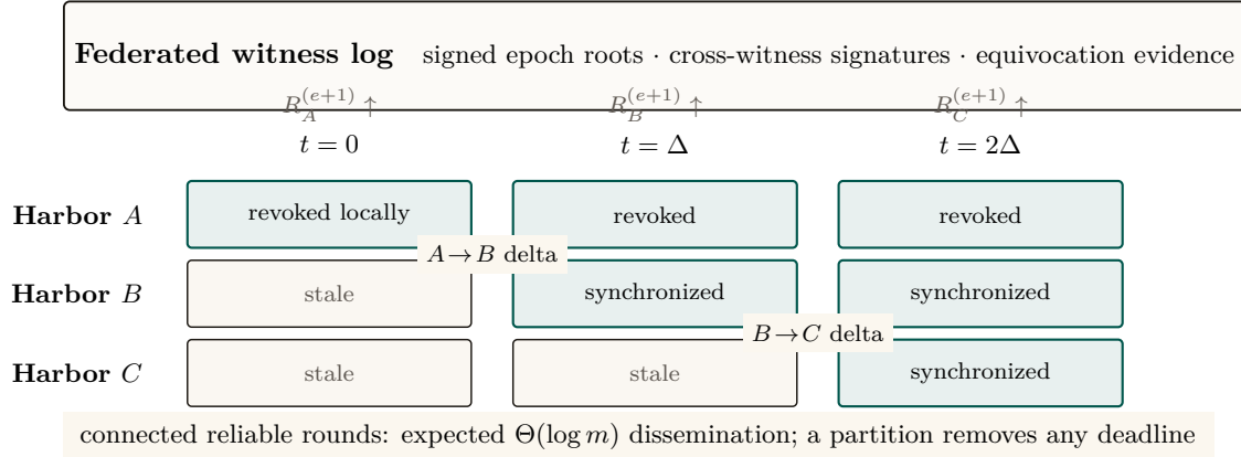
Figure 4: Revocation spreads epidemically in expected \Theta(\log m) rounds under the stated connected, reliable-round model. This is an expectation, not a worst-case deadline: an unbounded partition still yields unbounded exposure. Rows identify the authority whose local filter decides admission; columns expose the stale-verifier window. Signed per-epoch roots make contradictory histories auditable after delivery without pretending the federation has a global clock.
