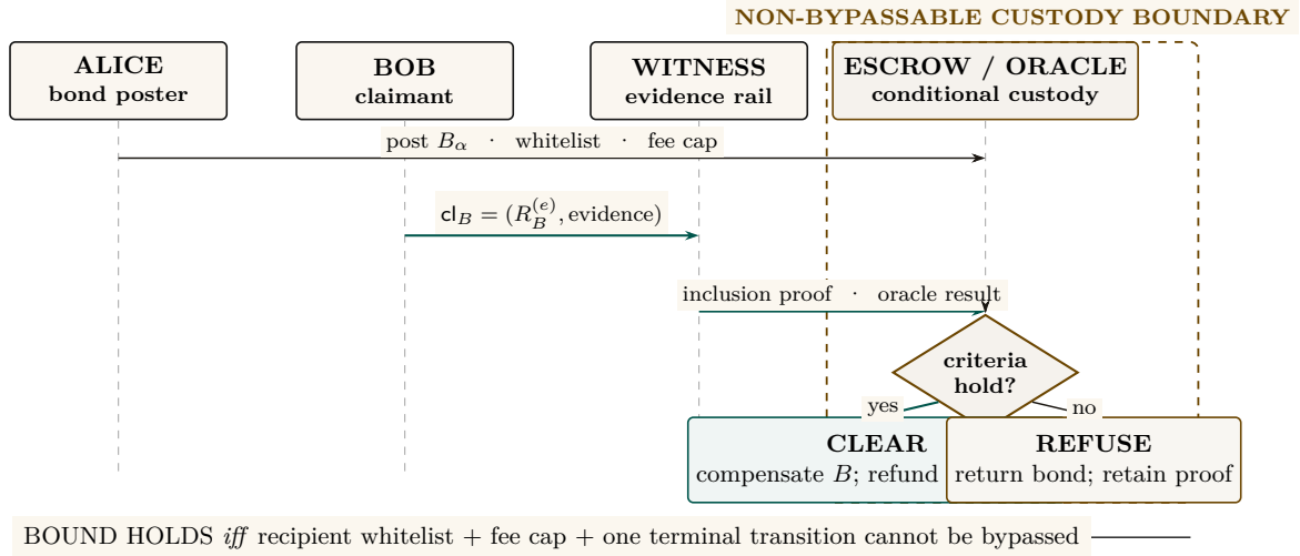
Figure 5: Cross-harbor settlement as an actor sequence with an explicit custody boundary. Alice posts the performance bond and its release constraints; Bob publishes a signed claim; the witness supplies the inclusion proof; only then may the escrow/oracle partition the outcome into Clear or Refuse . The custody bound remains conditional: Property 6.1 holds only where the recipient whitelist, fee cap, and single-terminal-transition rule cannot be bypassed by the escrow operator (§6.1).
