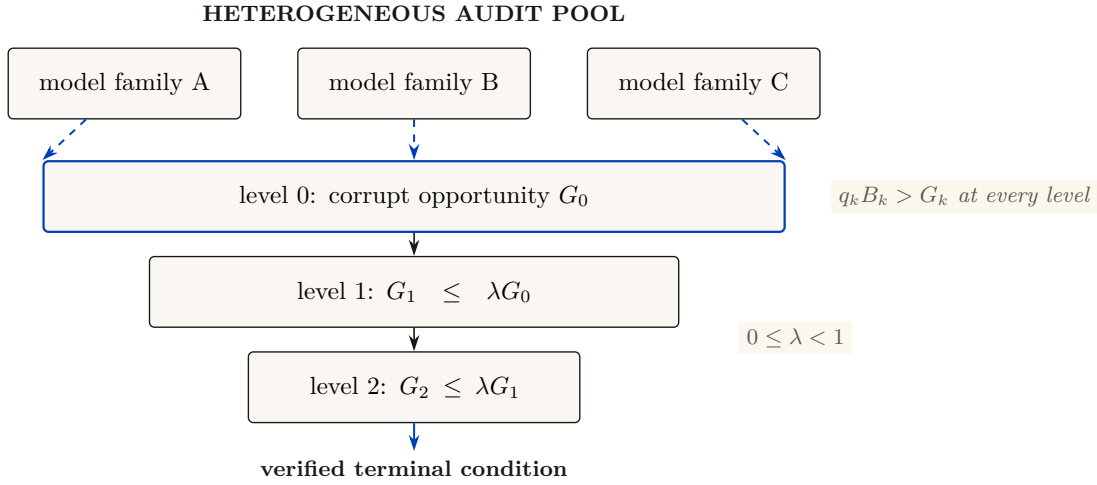
Figure 6: Recursive review terminates only if corruption opportunity contracts. Heterogeneous judge families reduce shared-mode failure, while each sampled level must satisfy both expected-forfeiture deterrence q_k B_k > G_k and a uniform contraction G_{k+1} \leq \lambda G_k . The narrowing geometry states the proof obligation; it does not depict the conjecture as established.
