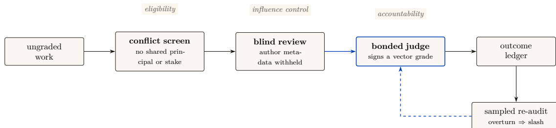
Figure 5: Neutrality is a gated ceremony. Work reaches a judge only after conflict screening and blind presentation; the selected judge posts a bond and signs the grade before it enters the outcome ledger. Sampled re-audit closes the loop by making an overturned grade costly to the judge itself.
