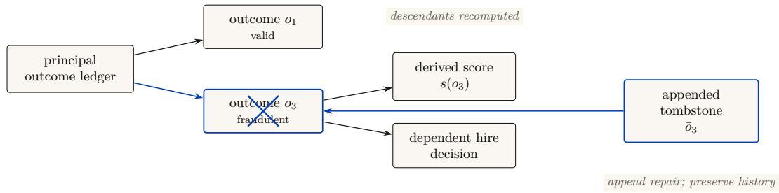
Figure 7: A tombstone invalidates a provenance branch without rewriting history. The fraudulent outcome remains in the append-only ledger, but the later tombstone marks it and every derived score or decision for recomputation. The protocol bounds the window during which descendants can rely on the poisoned entry; it does not pretend the window was zero.
