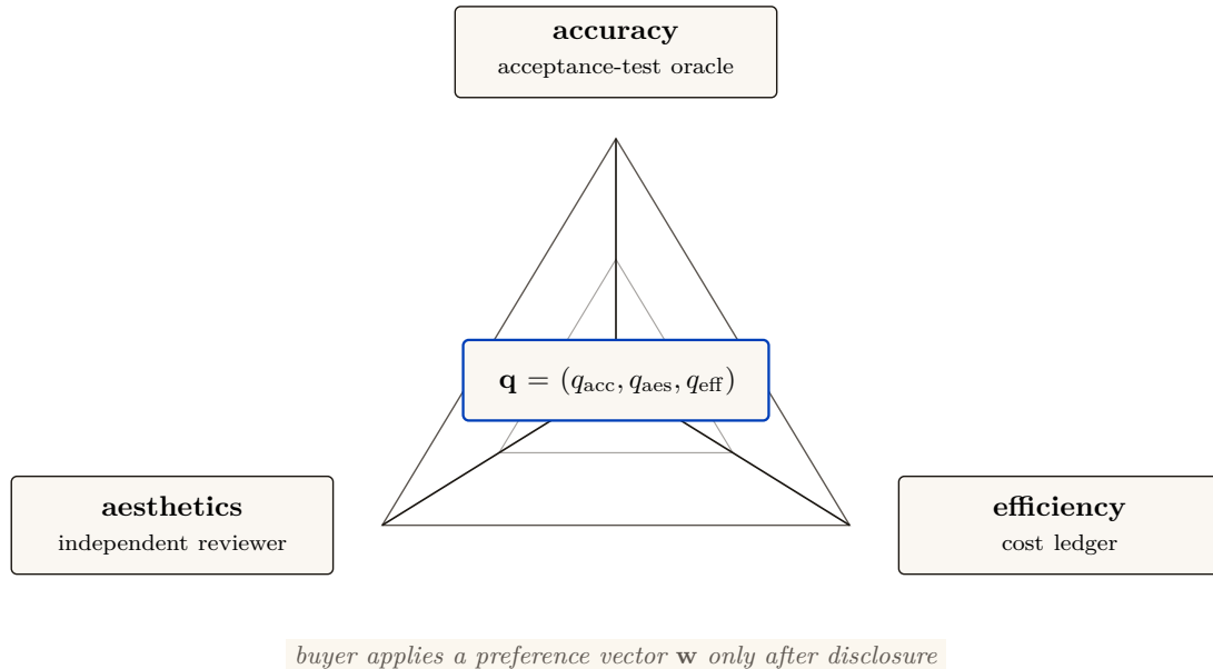
Figure 4: Quality remains a three-axis disclosure. Accuracy, aesthetics, and efficiency have different competent judges and cannot be collapsed without hiding trade-offs. The ledger publishes \mathbf{q} intact; each buyer then applies its own preference vector \mathbf{w} rather than inheriting a single Goodhart-able global score.
