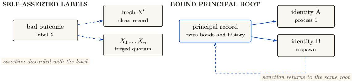
Figure 3: Identity binding determines whether sanctions survive churn. Self-asserted labels branch freely into a clean replacement or a forged quorum. With a daemon-minted identity bound to one economic principal, every descendant process returns outcomes and sanctions to the same durable root; respawning does not reset the ledger.
