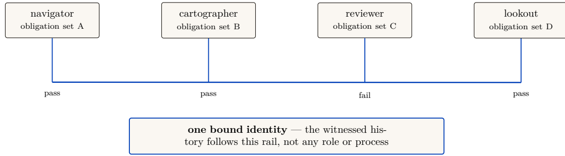
Figure 1: A person is the continuous provenance rail beneath changing roles. A role is fillable and history-free; each process may occupy a different role instance. Outcomes accumulate against one bound identity, so reputation survives role changes and respawns without being attached to an org-chart slot.
