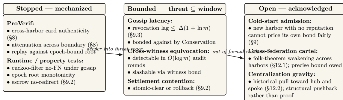
Figure 10: Threat-band layout for the Federated Harbor. The Anchor paper’s defense-in-depth structure carries over: every claim either has a mechanization artifact (sage), a named bound that the bond can price against (brass), or an explicit acknowledgement of the open frontier (cinnabar). The paper is disciplined about which band each claim lives in — see Appendix A for the artifact registry. Bands shift left over time as future work mechanizes what is presently bounded.
