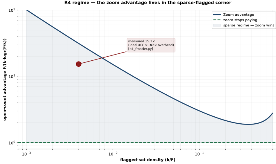
Figure 6: Regime diagram for the zoom advantage: the idealized open-count advantage F/(k \log_2(F/k)) against flagged-set density k/F , over the sparse-to-moderate range this digest architecture targets. The advantage is steep where flags are sparse ( k \ll F ) and falls toward parity as density grows; the plotted idealization never crosses parity, but the deployed algorithm’s constant overhead does invert the ordering at higher density still, exactly as measured at (F, k) = (100, 90) in §5.2 (199 adaptive opens against 100 flat) — both halves of the claim are load-bearing.
