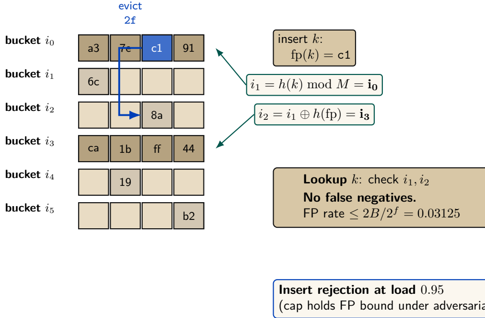
Figure V.5: Cuckoo-filter revocation gate (Fan et al. [35]) with the load-factor ceiling that defeats the pollution attack. Insert lands at either of two candidate buckets i_1, i_2 = i_1 \oplus h(fp) ; on full, evict and re-insert at the kicked fingerprint’s alternate. Insert rejection at 0.95 caps occupancy inside the regime where the false-positive bound holds.
