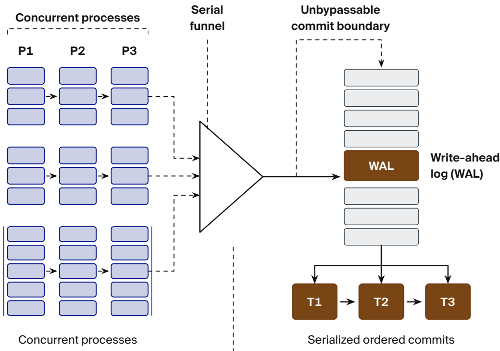
Figure 0.1: Proposition 1 Mechanics: Serial Write Arbitration. Parallel, uncoordinated writer attempts from independent agent processes ( P_1, P_2, P_3 ) funnel through an unbypassable commit boundary into a single serialized write-ahead log (WAL). Mutations receive a strict total causal order ( T_1 \rightarrow T_2 \rightarrow T_3 ), eliminating physical race conditions and lost updates at the effect boundary.
