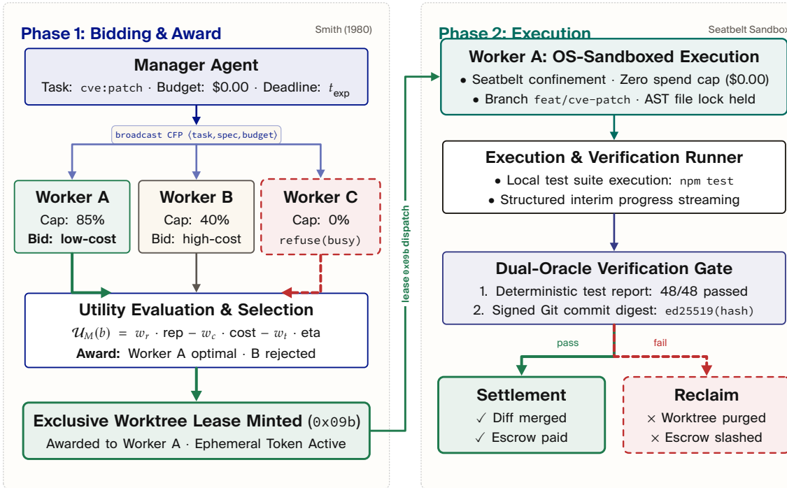
Figure 0.12: Contract Net Protocol (CNP) Task Allocation Lifecycle and Settlement Under Kernel Confinement. Grounded in Reid Smith’s (1980) bilateral market protocol. Phase 1 (left): Manager agent broadcasts a Call for Proposals (CFP) with task specification and spend cap; eligible contractors evaluate tool capacity and submit bids, or return explicit refusals under lock contention. Phase 2 (right): Winning contractor receives an exclusive worktree lease (0x09b), executing inside a Seatbelt sandbox under a zero-spend cap. Escrow funds unlock strictly upon presentation of signed git commit hashes and cryptographic test run receipts.
