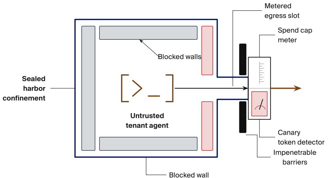
Figure 0.3: Proposition 3 Mechanics: Sealed Room Confinement. Operating system sandbox profiles (Seatbelt SBPL / Linux Landlock) enclose untrusted agent subprocesses, severing ambient network and shared disk paths. All outbound communication must traverse a single metered egress slot governed by canary token inspection and conserved spend caps.
