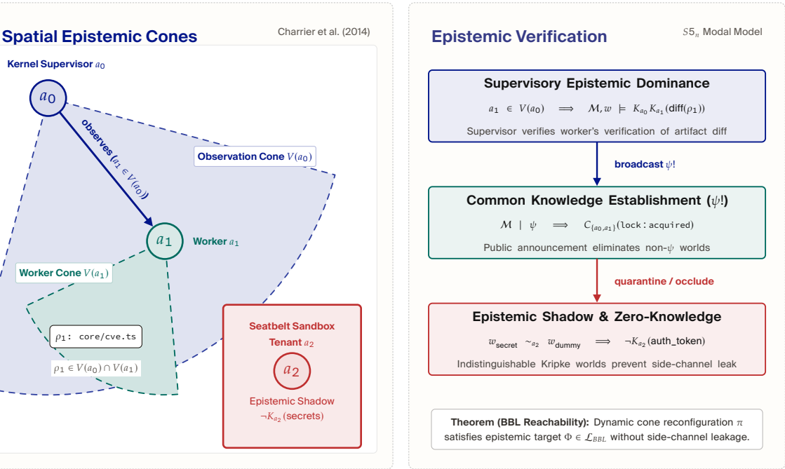
Figure 0.13: Dynamic Epistemic Observation Cones in Big Brother Logic (BBL) (Charrier et al., 2014). Directed vision cones formalize asymmetric visibility, epistemic shadows, and higher-order knowledge verification ( K_{a_1} K_{a_2} \phi ) in autonomous multi-agent systems. The supervisor maintains epistemic dominance over worker mutations, while sandboxed tenants operate within strict epistemic shadows, preventing side-channel data exfiltration.
