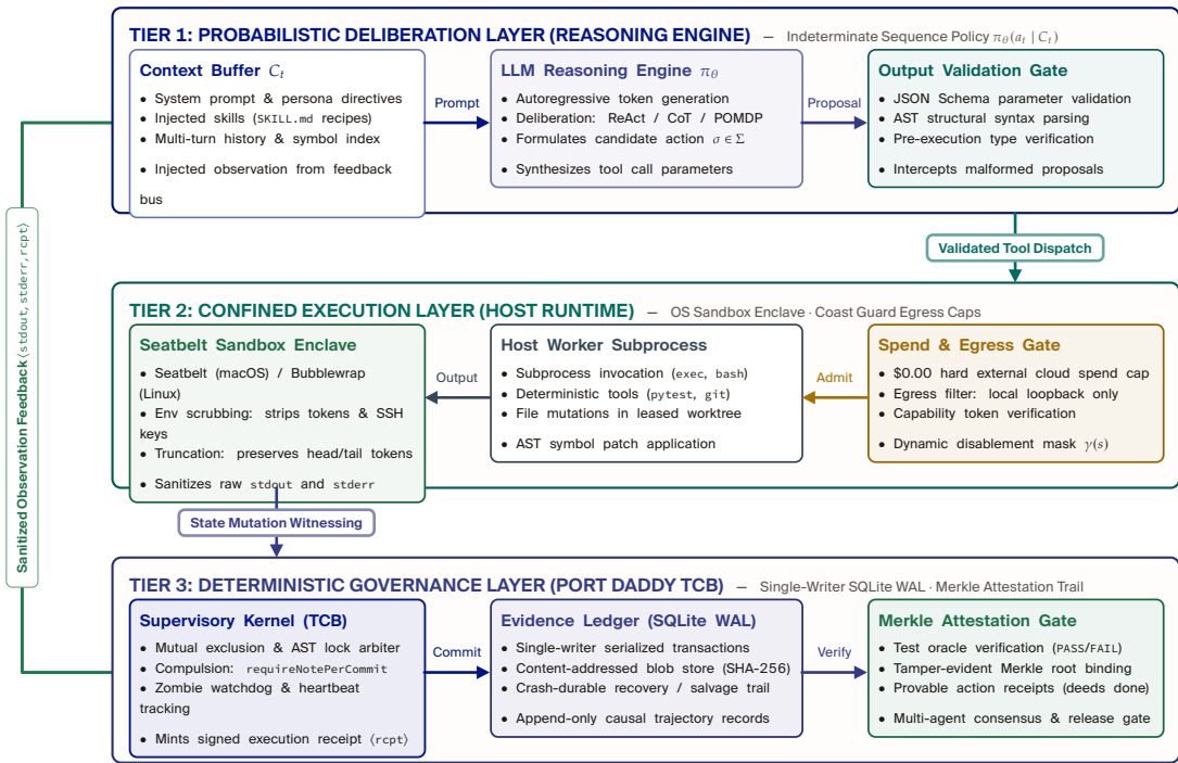
Figure 0.18: The Closed Agentic Architecture Loop. Three architectural tiers separating probabilistic deliberation from deterministic kernel coordination: (1) Probabilistic Deliberation Layer (LLM reasoning and planning); (2) Confined Execution Layer (sandboxed host containers and tool execution); and (3) Deterministic Governance Layer (single-writer SQLite WAL, capability verification, and tamper-evident Merkle attestation).
