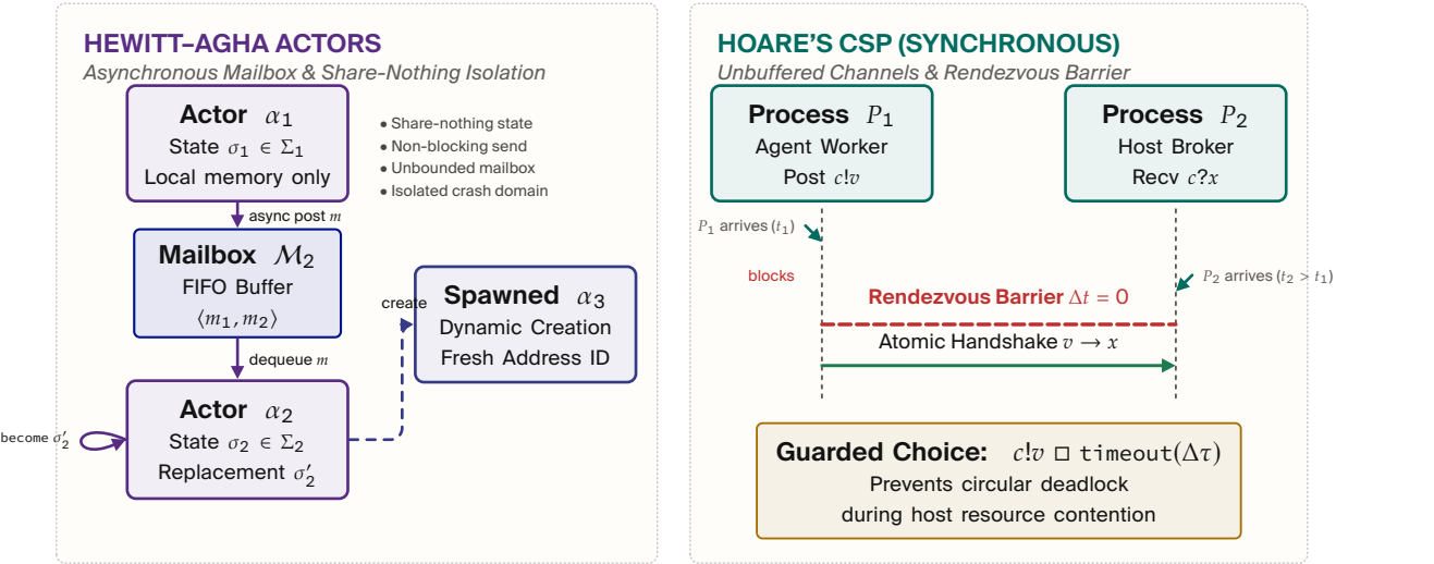
Figure 0.10: Concurrency Foundations for Multi-Agent Operating Kernels. Synthesizing Hewitt-Agha virtual actor isolation (asynchronous mailboxes, capability tokens, and become state transitions) with Hoare’s Communicating Sequential Processes (synchronous rendezvous barriers, \Delta t = 0 , and guarded external choice with lease timeouts). Sovereign actors deliberate in isolated sandboxes, while physical host resource contention (TCP ports, SQLite WAL writes, mutex locks) is arbitrated via synchronous CSP rendezvous.
