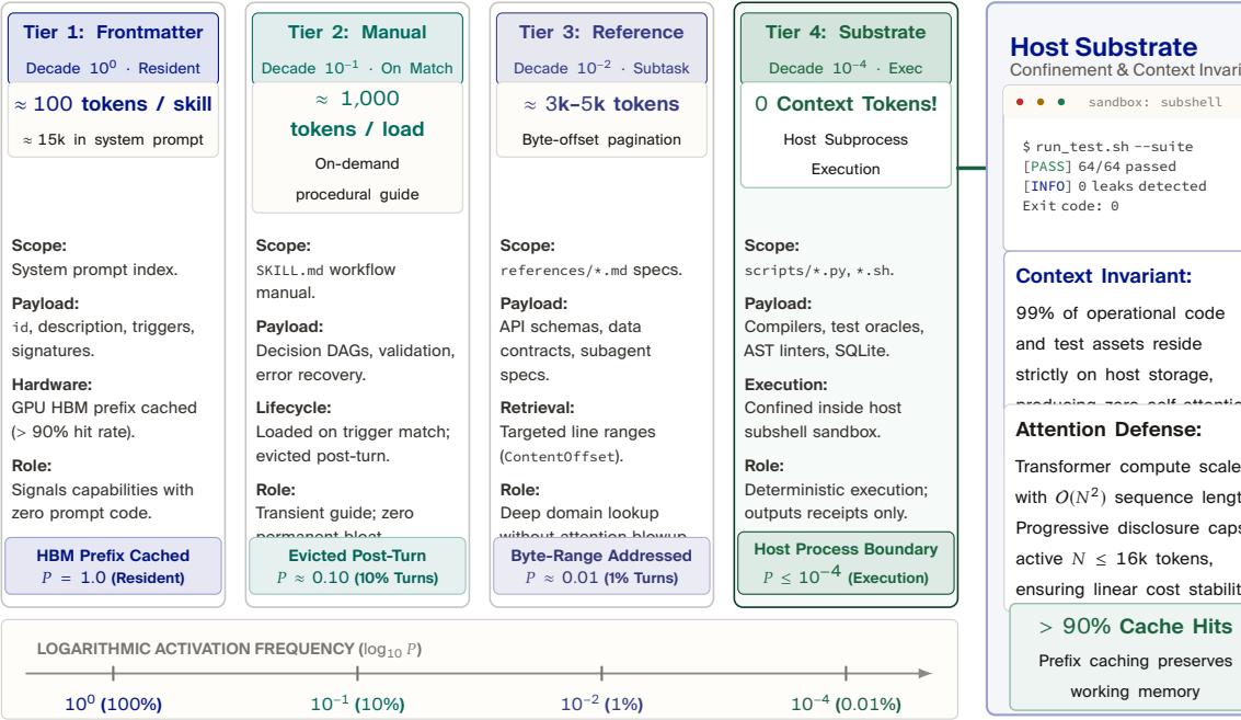
Figure 0.15: Progressive Disclosure of Skills Across Contracting Logarithmic Decades. Capability activation frequency contracts across decades ( 10^0 to 10^{-4} ). By partitioning capabilities from static frontmatter metadata down to host-executed scripts and formal schemas consuming zero LLM context tokens, context consumption contracts exponentially with task specialization.
