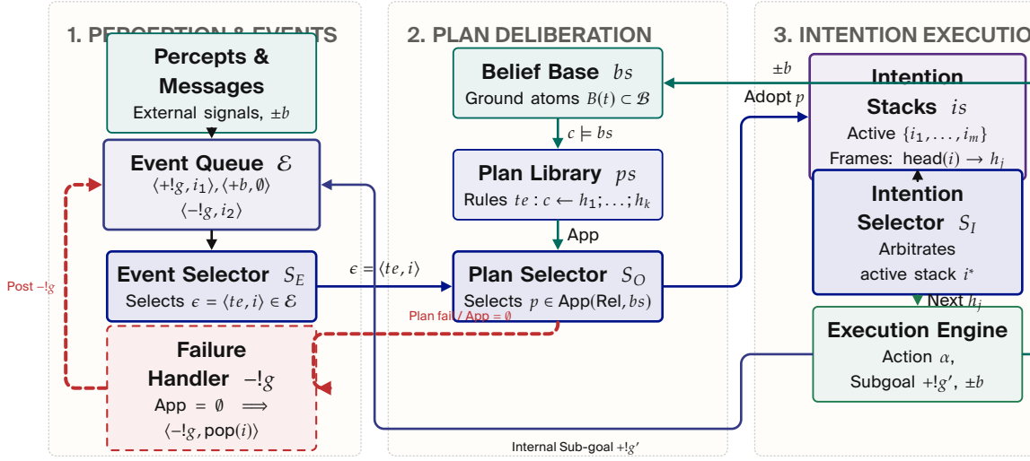
Figure 0.9: BDI Execution Flow and Operational Choice Architecture. Grounded in real world software engineering workflows, adapted from AgentSpeak(L) semantics (Bordini et al. 2007). Contrasting reactive rule triggers, static STRIPS-style planners, and dynamic BDI agents. The three core selection functions ( S_E for events, S_O for applicable plans, and S_I for intention stacks) arbitrate runtime goal scheduling, with explicit plan failure handling via the -!g recovery event.
