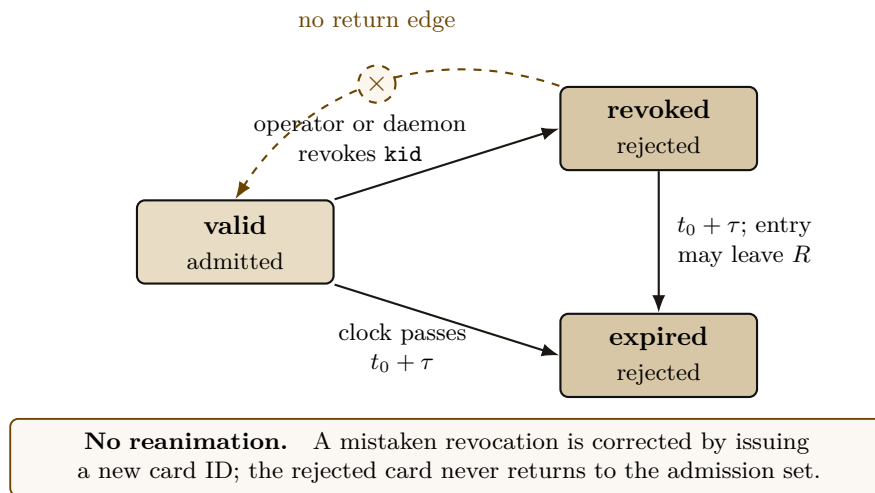
Figure 7: The Harbor Card lifecycle. A card leaves the valid state in exactly two ways — an explicit revocation, or the clock reaching t_0 + \tau — and returns from neither. The crossed dashed arrow is the figure’s actual claim: the revoked \rightarrow valid transition is absent by design (Property 2.3), not merely undrawn. After expiry the entry may be dropped from the revocation log R without weakening anything, because the card is already unacceptable on its exp claim alone.
