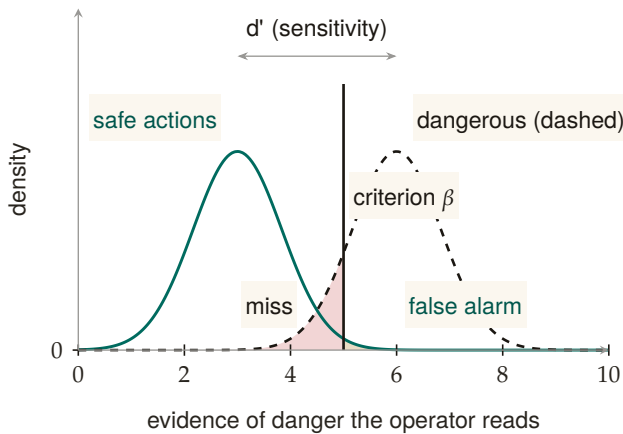
Figure 4.5: The operator’s forced-zoom decision as Signal Detection Theory (Def. 4.5.1). Two named densities over the evidence the operator reads: safe actions (solid) and dangerous actions (dashed), separated by sensitivity d' . Zooming triggers when evidence exceeds the criterion \beta ; moving \beta left trades the caution-tinted miss region for more of the neutral-tinted false-alarm region. Because a miss costs far more than a false alarm — at the chapter’s running costs, 100 against 5, the inspect bar sits at a \geq 0.057 — the optimal criterion sits well to the left of the throughput optimum: idealized as two fixed Gaussians, not the fitted mixture the deployed detector would use [internal].
