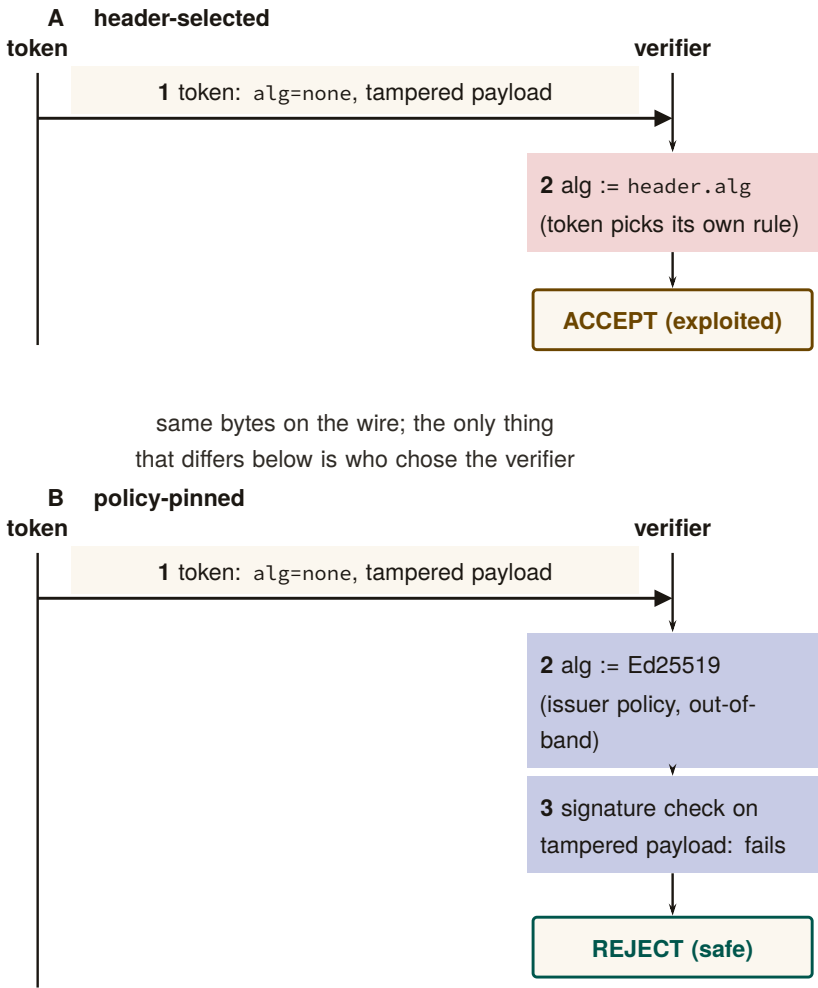
Figure 2.3: Two verifier ladders for the same wire bytes: token sends alg=none with a tampered payload to verifier in both panels. Panel A lets the token’s own header choose the algorithm and message 2 accepts the forgery; panel B pins the algorithm to Ed25519 from issuer policy, so message 3’s signature check fails and the token is rejected. This is the design invariant behind the ProVerif v1 (HS256) query \neg \text{attacker}(\text{master\_key}) \text{ holding TRUE} : the accepting path in panel A is exactly the path Algorithmic Pinning removes [verified, v1_refined.pv].
