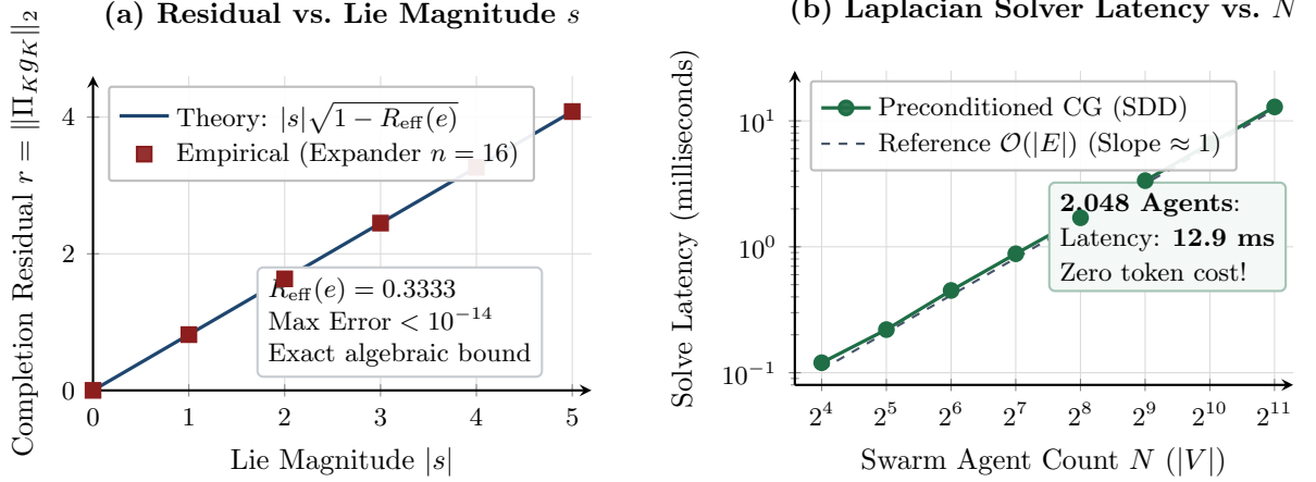
Figure 6: Numerical verification of Theorems CR-1 through CR-3 on synthetic expander meshes. (a) Observed residual r against lie magnitude s on a 16-agent mesh ( R_{\text{eff}} = 1/3 ), confirming the closed form r = |s|\sqrt{1 - R_{\text{eff}}(e)} with relative error < 10^{-14} . (b) Empirical solve latency of SDD Laplacian preconditioned CG solver from N = 16 to N = 2,048 agents, confirming near-linear scaling ( \sim 12.9 ms at 2,048 nodes).
