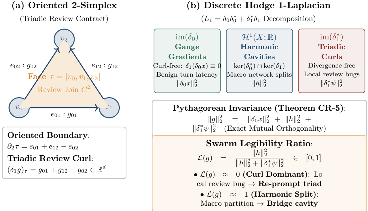
Figure 4: Discrete Hodge decomposition on a simplicial 2-complex. (a) A 2-simplex \tau = [v_0, v_1, v_2] modeling a 3-way review contract with oriented boundary \partial_2 \tau = e_{01} + e_{12} - e_{02} . (b) The Hodge 1-Laplacian L_1 = \delta_0 \delta_0^* + \delta_1^* \delta_1 decomposes observed discrepancies into mutually orthogonal gauge gradients, harmonic cavities, and triadic curls, providing the zero-token Swarm Legibility Ratio \mathcal{L}(g) .
