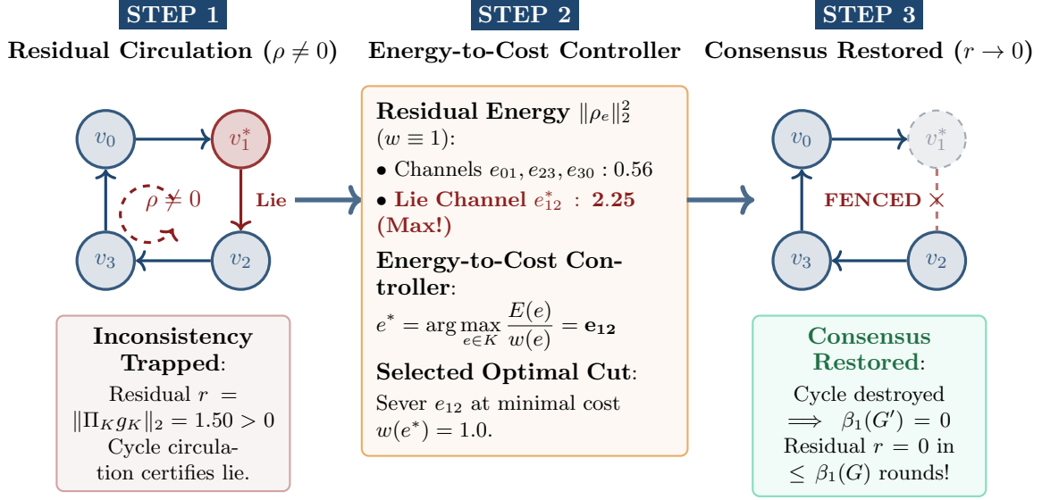
Figure 5: Theorem CR-4 active repair closed loop. (Step 1) An equivocator v_1^* injects contradiction s = 3.0 , creating non-zero circulation \rho \neq 0 . (Step 2) The greedy controller computes residual energy-to-cost ratios E(e)/w(e) across active channels. (Step 3) Severing optimal edge e_{12}^* breaks the cycle constraint, restoring consensus ( r \rightarrow 0 ) in polynomial time.
