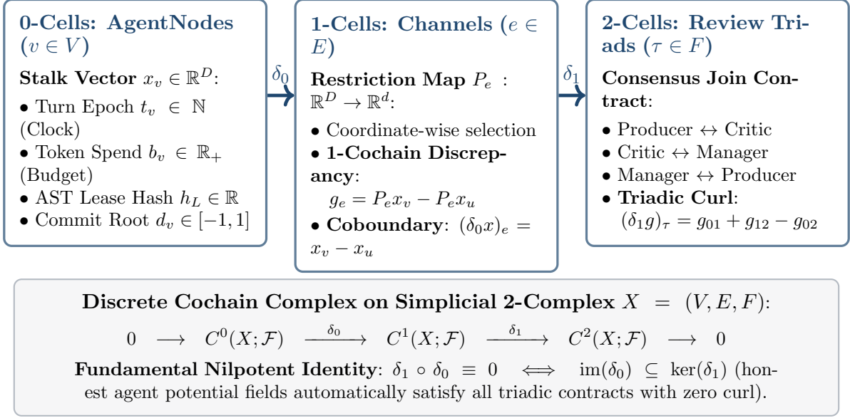
Figure 3: The Rosetta Stone: exact algebraic translation from multi-agent swarm primitives into cellular sheaves and simplicial complexes over cell complex X = (V, E, F) .
