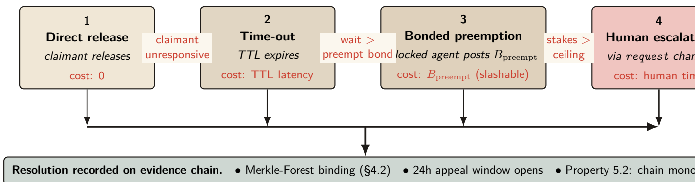
Figure 1: Governance and appeals: four-stage escalation path. The daemon resolves most disputes at step 1 or 2 (zero or near-zero cost). Bonded preemption (step 3) prices the blocked agent’s claim that the holder is wrong; if the preemption is wrong, the bond is slashed under settlement. Human escalation (step 4) is reserved for the cases the daemon cannot mechanically decide. Every resolution is appended to the evidence chain with the same Merkle-Forest binding as any agent action, so all four stages remain auditable.
