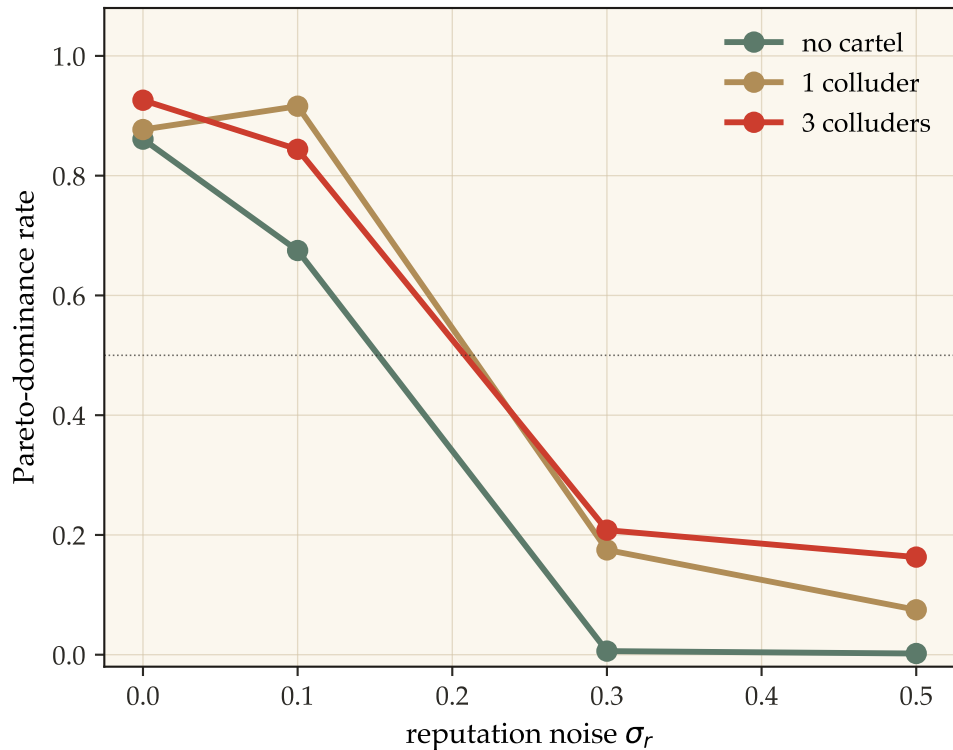
(a) dominance rate vs \sigma_r ( n = 5 )
