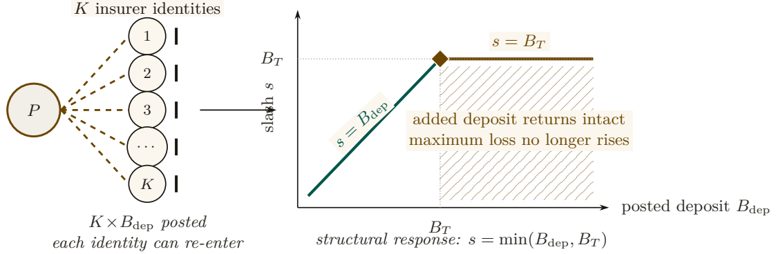
Figure 3: Deposit-only Sybil deterrence saturates. One principal can fund K interchangeable identities, but the loss attached to a defaulting identity rises only until its deposit reaches the transaction coverage B_T . Past that knee, s = \min(B_{\text{dep}}, B_T) = B_T : additional posted capital returns intact on no-loss transactions and cannot increase the attacker's maximum loss. Figure 4 shows the corresponding simulated profit and commons-deficit sweeps.
