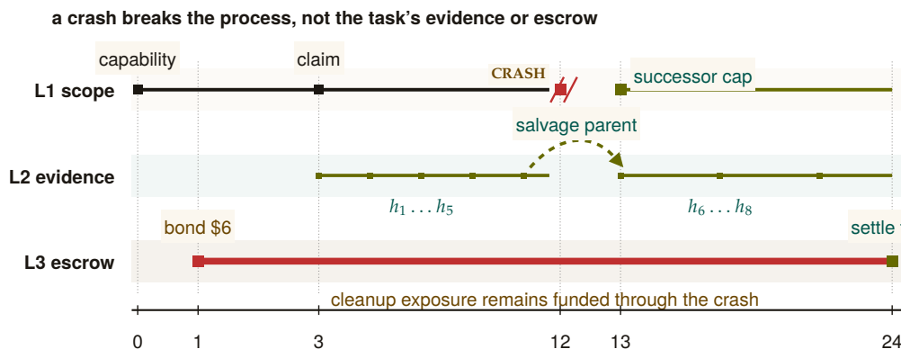
Figure 7.10: The worked example is a continuity braid over one task. Structural authority belongs to a process and visibly breaks at minute 12; the successor receives a new capability at minute 13. The evidence chain does not break: its salvage-parent edge binds h_1 \dots h_5 to h_6 \dots h_8 . The escrow rail spans the entire task and settles at minute 24. Identity is disposable, while attribution and pre-funded cleanup exposure persist.
