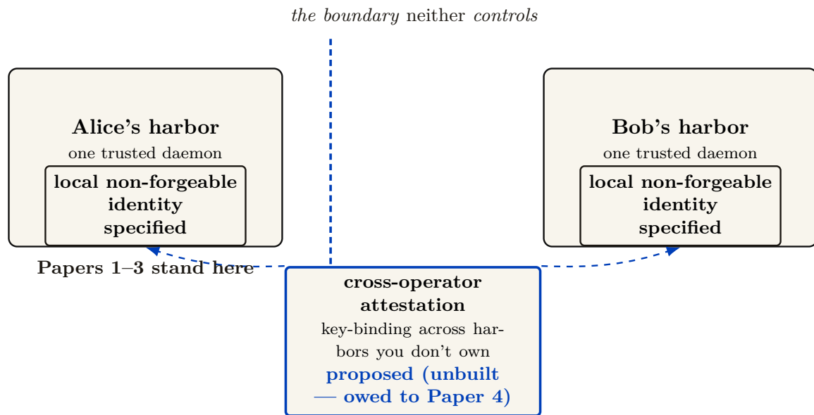
Figure 7: The keystone is two stones. A local non-forgeable identity secures identity within one trusted daemon — exactly what Papers 1–3 need and assume. The cross-operator boundary needs cross-operator attestation , which is unwritten — a federated witness log gives log- integrity , not identity- binding . This paper depends on the solid stone and hands the market paper the unbuilt one by name , rather than borrowing the single-operator threat model across the boundary.
