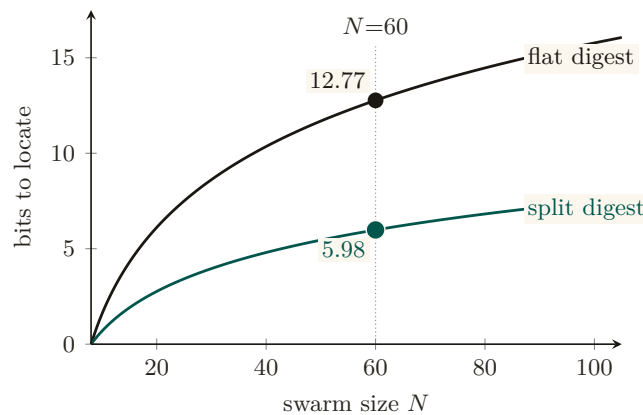
Figure 6: Bits an operator must read to locate the critical artifact, at the lower bound of Thm. 6.1 with m=8 , k=2 . One flat digest serving both readers jointly needs \text{Floor}(N, 4, 8) bits; two split digests, one per reader, each need only \text{Floor}(N, 2, 8) . At N=60 the split digest costs 5.98 bits against the flat digest’s 12.77 — a 2.13\times penalty, not the 2\times that halving the readers would predict. The committed sweep CSV ( r1-floor.csv ) is not yet present, so the two curves are the chapter’s own closed-form Floor formula rather than simulated points; only the N=60 values it works by hand are marked [internal].
