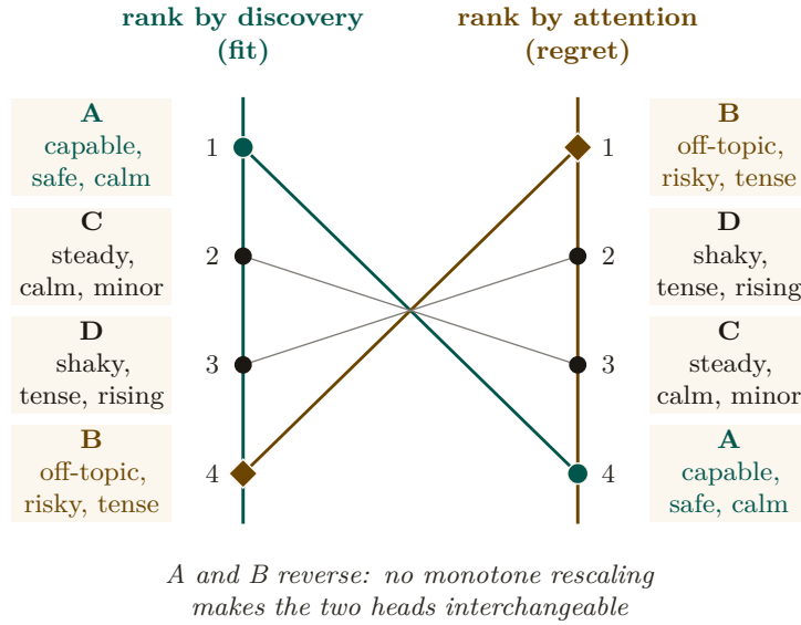
Figure 7: One candidate pool under two loss functions, ranks 1–4 on both axes. Discovery ranks by fit; attention ranks by expected regret if ignored. Candidate A is the best fit but safest to skip, while B is a poor fit but the most dangerous to miss, so their ranks fully invert (1–4 against 4–1). C and D swap one adjacent pair, the same non-comonotone fact at smaller scale. Shared candidate generation and recency decay do not make the two scoring heads interchangeable [internal].
