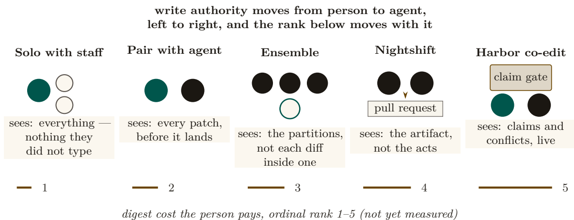
Figure 5: The chapter’s five modes of cooperation, ordered by how much write authority has left the person: a filled circle holds write authority, a hollow circle only observes. Solo with staff changes nothing the person did not type; Pair with agent splits authority turn by turn; Ensemble distributes it by partition, so the tracking person sees the partitions rather than every diff; Nightshift hands agents unattended write authority inside a budget and shows the person only the resulting artifact; Harbor co-edit restores co-equal authority but gates same-symbol writes through a claim lock. The bar under each panel is an ordinal rank, not a measured cost — the front matter names the study that would measure it. [internal]
