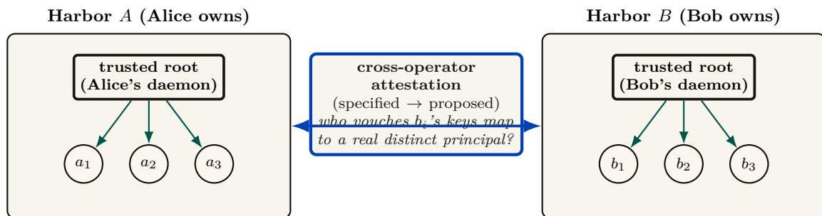
Figure 4: The keystone split. Chapters I–III rest on local non-forgable identity : a per-agent identity no agent can edit within one trusted daemon — a single trusted root that vouches for every agent it mints. That is exactly what a single-operator harbor needs. But the market is defined by mutually-distrusting operators trading across a boundary neither controls, and that primitive explicitly disclaims the relevant threat model (intra-fleet, not a cross-party PKI, no hostile-operator defense). Binding signing keys across harbors you do not own is a different, unsolved problem: cross-operator attestation . Across the boundary, the counterparty’s daemon is the adversary the local threat model declares out of scope, and the witness log gives log integrity , not identity binding . It is the highest-leverage unbuilt keystone, and it gates the entire market thesis.
