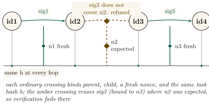
Figure 3: The delegation chain as a signed provenance braid across four identities id1–id4. Ordinary hops 1 and 3 bind parent, child, a fresh nonce (n1, n3), and the shared task hash h; the shared task hash h below. Hop 2 shows a splice attack: an attacker moves the legitimate signature sig3 (computed over id3, id4, and n3) into the id2–id3 position, where the verifier expects a signature over n2; the check fails at exactly that crossing, so the discontinuity is visible at one adjacent-identity boundary rather than anywhere else in the chain. [internal]
