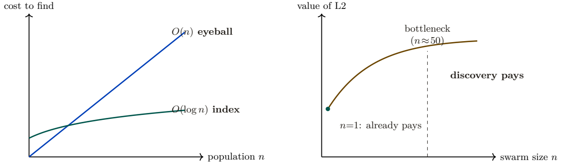
Figure I.7: Read-poverty (§I.6): state piles up faster than it can be read. Left: the cost of finding the right agent/work grows linearly under eyeball search but stays near-flat under an indexed directory — the same trade every database made at the table-scan wall. Right: the value curve of the legibility wedge across swarm size. It is valuable already at n=1 (briefing, attestation, footgun guard, honest completion) and grows into the read-poverty regime; discovery ranking earns its keep around the n \approx 50 bottleneck. The wedge must work at n=1 and grow gracefully.
