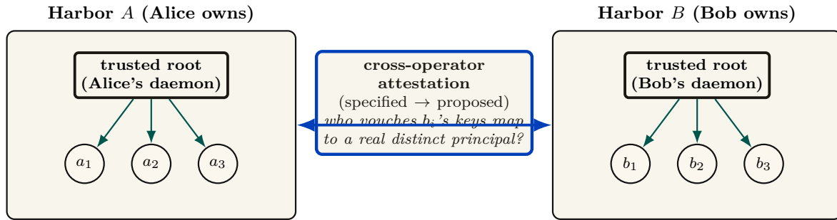
Figure IV.4: The keystone split. Chapters I–III rest on local non-forgeable identity : a per-agent identity no agent can edit within one trusted daemon — a single trusted root that vouches for every agent it mints. That is exactly what a single-operator harbor needs. But the market is defined by mutually-distrusting operators trading across a boundary neither controls, and that primitive explicitly disclaims the relevant threat model (intra-fleet, not a cross-party PKI, no hostile-operator defense). Binding signing keys across harbors you do not own is a different, unsolved problem: cross-operator attestation . Across the boundary, the counterparty’s daemon is the adversary the local threat model declares out of scope, and the witness log gives log integrity , not identity binding . It is the highest-leverage unbuilt keystone, and it gates the entire market thesis.
