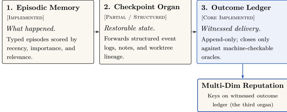
Figure III.4: The three continuity organs, formally classified. Episodic Memory records what happened (typed episodes promoted out of transient history). The Checkpoint Organ preserves task lineage and worktree state across compaction boundaries. The Witnessed-Outcome Ledger enforces non-repudiable delivery against external oracles, serving as the sole cryptographic anchor for multi-agent reputation.
