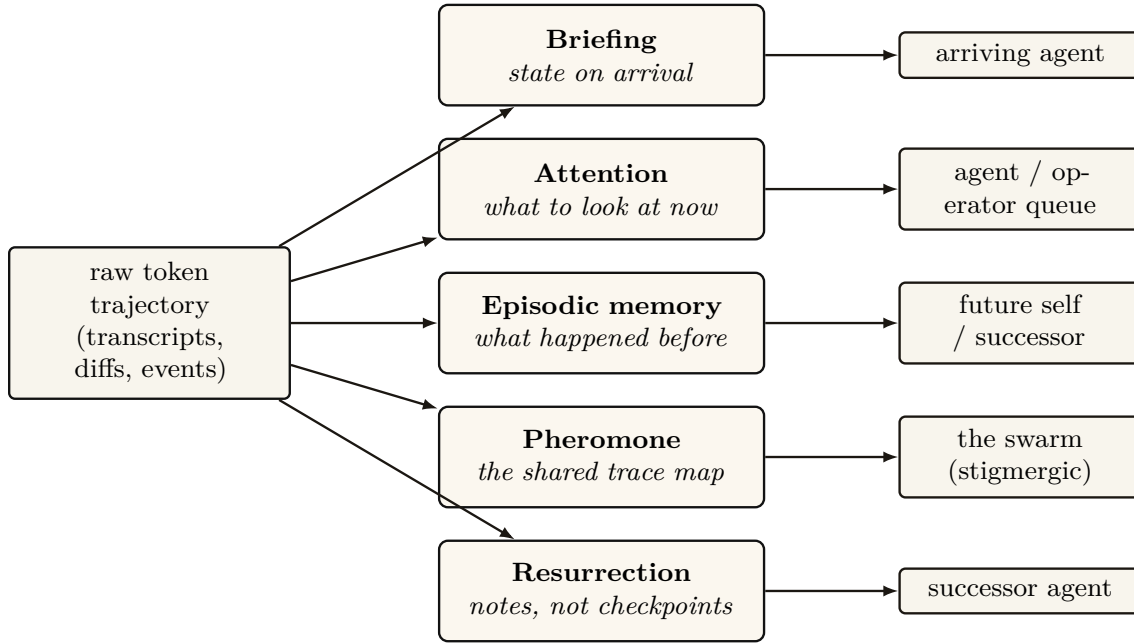
Figure I.9: Five read-surfaces, each a token-compaction of the raw trajectory produced for a specific reader (§I.8.2): briefing is external note-taking, attention is precision compaction, episodic memory is recall-then-precision, pheromone is time-decay (forgetting), resurrection is a handoff summary. Viewed correctly, the swarm’s coordination layer is a distributed compaction engine — and because each surface is a compaction, each is governed by the same cost-and-legibility economics, the same recency-decay (Prop. I.7.1), and the same one law (Def. I.3.1).
