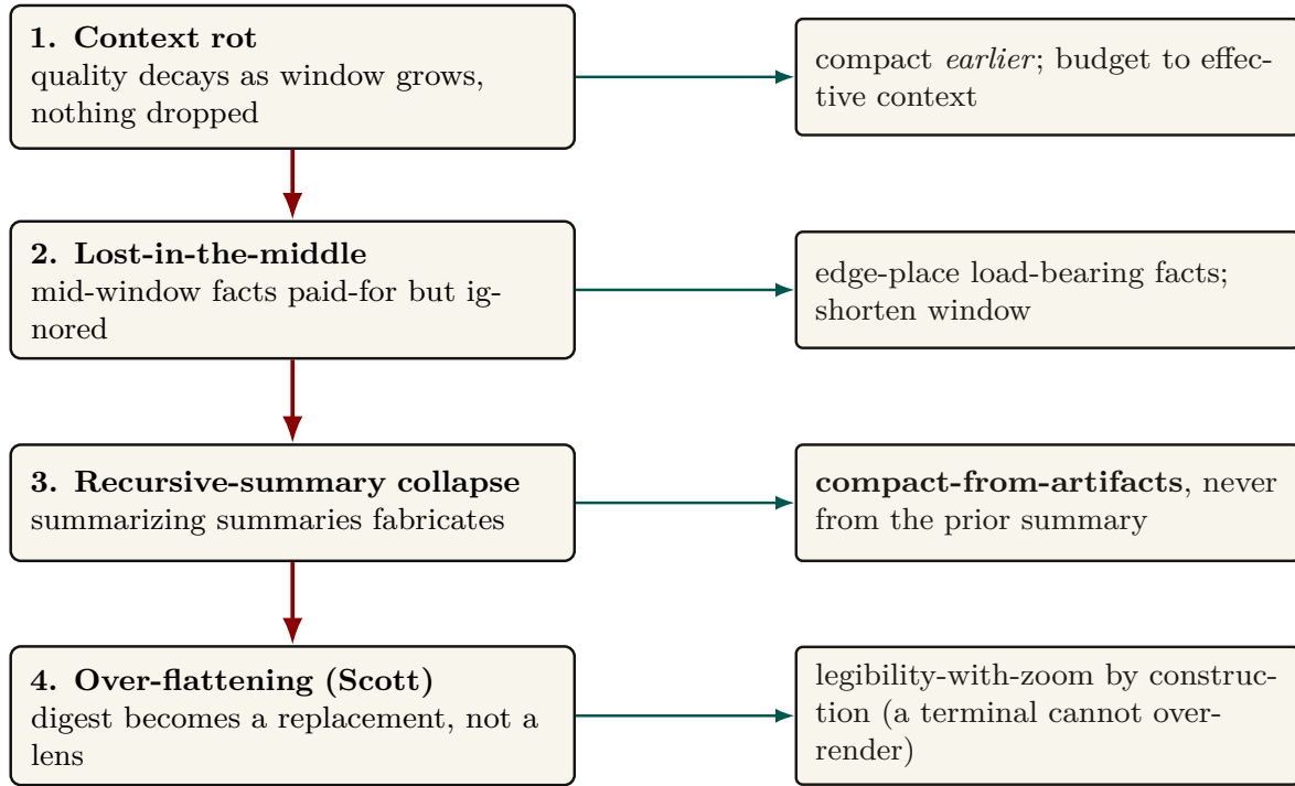
Figure I.10: The context-degradation cascade (§I.8.3): rot makes you compact, naive compaction loses the middle, recursion fabricates, and the operator-facing digest over-flattens what’s left — the failures compound, hence “cascade.” Each rung (red) has a cure (teal), and breaking any rung stops the cascade; the load-bearing cure is compact-from-artifacts (rung 3), which a system with durable, addressable state (claims, notes, episodes) makes cheap. Cost and legibility share this surface: when compaction fails, the bill and the truth degrade together.
