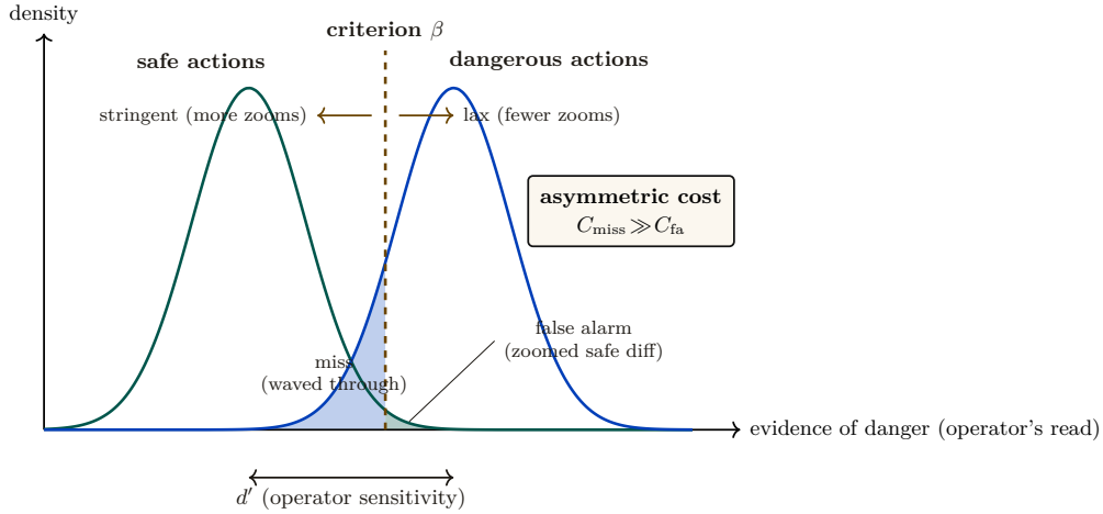
Figure I.6: The operator’s forced-zoom decision as Signal Detection Theory (Def. I.5.1, Eq. I.1). Most actions are safe (left curve); a few are dangerous (right). Zooming triggers when evidence of danger exceeds criterion \beta . Moving \beta left is more stringent: it causes more zooms, fewer misses, and more false alarms. Moving \beta right is more lax: it minimizes attention-seconds but increases misses. Because C_{\text{miss}} \gg C_{\text{fa}} , the optimal criterion sits well to the left of the throughput optimum: the miss-cost term is what forces the zoom . Sensitivity d' (curve separation) is improved by better legibility; \beta is the policy knob p(r, s, v) .
