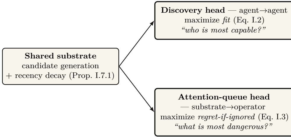
Figure I.8: The split ranker (Thm. I.7.1). The discovery ranker and the operator’s attention queue share candidate generation and recency-decay (Prop. I.7.1) over the same signals — claims, skills, notes, episodes, presence — but apply distinct scoring heads: discovery maximizes fit (capability match, Eq. I.2); the attention queue maximizes regret-if-ignored (Eq. I.3). The operator wants the most dangerous item surfaced, the agent wants the most capable collaborator — incompatible loss functions, not one objective with swapped weights, so the elegant “one ranker” claim is false-as-stated and demoted to “shared substrate, distinct heads.”
