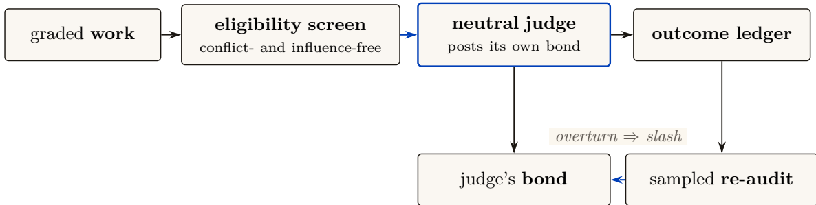
Figure III.11: The neutral-judge market. Graded work flows to a judge selected for conflict- and influence-freedom; the judge posts its own bond, the grade enters the outcome ledger, and a sampled re-audit can slash a judge whose grade is overturned. “Neutral” is a checklist (conflict-free, influence-free, de-biased), not a vibe, and the judge is hired through the same bonded ceremony the market uses for any task (Protocol III.10.1) — the judge’s own reputation is the asset it protects.
