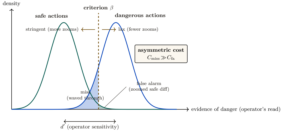
Figure 6: The operator’s forced-zoom decision as Signal Detection Theory (Def. 5.1, Eq. 1). Most actions are safe (left curve); a few are dangerous (right). Zooming triggers when evidence of danger exceeds criterion \beta . Moving \beta left is more stringent: it causes more zooms, fewer misses, and more false alarms. Moving \beta right is more lax: it minimizes attention-seconds but increases misses. Because C_{\text{miss}} \gg C_{\text{fa}} , the optimal criterion sits well to the left of the throughput optimum: the miss-cost term is what forces the zoom . Sensitivity d' (curve separation) is improved by better legibility; \beta is the policy knob p(r, s, v) .
