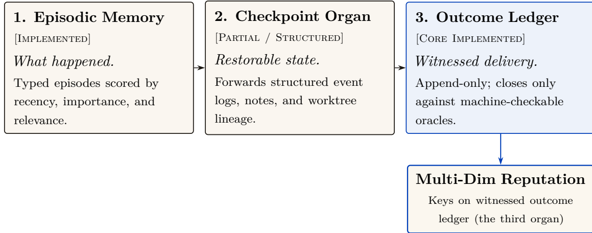
Figure 4: The three continuity organs, formally classified. Episodic Memory records what happened (typed episodes promoted out of transient history). The Checkpoint Organ preserves task lineage and worktree state across compaction boundaries. The Witnessed-Outcome Ledger enforces non-repudiable delivery against external oracles, serving as the sole cryptographic anchor for multi-agent reputation.
