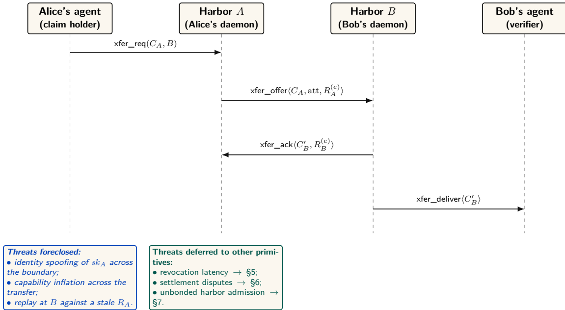
Figure 3: The four-message cross-harbor capability transfer ceremony. The critical property is that no message after (3) needs to reach back to Harbor A in the hot path: C'_B is verifiable under sk_B alone, which is why federation does not turn every authorization into a synchronous inter-machine round trip. The epoch root R_A^{(e)} bound into the envelope is the load-bearing primitive — a revocation issued by A after epoch e invalidates C'_B as soon as the new R_A^{(e+1)} reaches the witness log that B audits.
