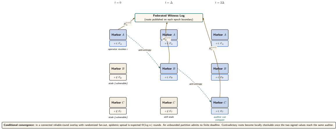
Figure 4: Federated revocation propagation across three harbors. The cuckoo filter mechanism is unchanged from Anchor §2.4 of the companion paper, but two new pieces are bolted on: (a) per-epoch roots R_X^{(e)} published to a shared witness log so a third party can audit any harbor’s local view, and (b) cross-witness signatures so the auditor pattern generalizes Certificate Transparency [9]. The illustrated \Delta -spaced hops are one execution, not a universal deadline: availability depends on overlay connectivity and delivery assumptions.
