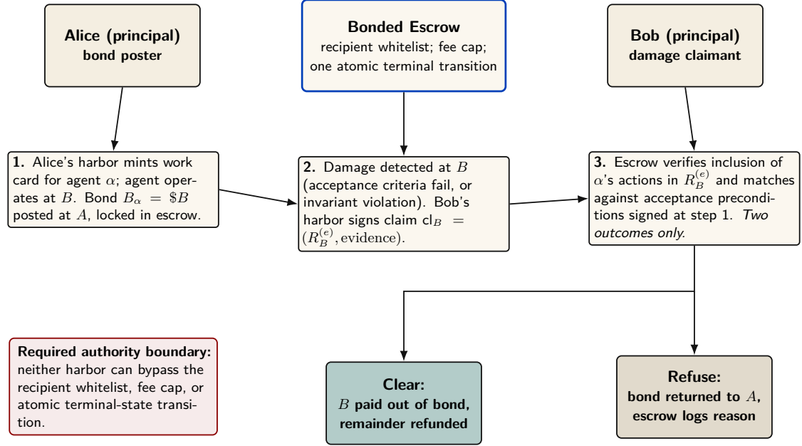
Figure 5: Cross-harbor settlement protocol. The custody bound is conditional, not automatic: the escrow authority must enforce a recipient whitelist, a fee cap, and exactly one atomic terminal transition, and neither harbor may possess an out-of-band bypass. Under those assumptions the outcome space is clear or refuse. Without them, the worst-case loss is the full balance held in custody.
