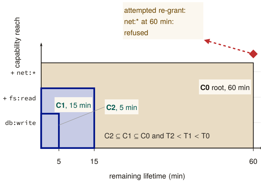
Figure 2.1: Nested rectangles for the capability envelope C0 (root, 60 min), C1 (15 min) and C2 (5 min): each child rectangle sits strictly inside its parent on both axes. The amber datum is an attempted re-grant of \text{net}:* at the full 60-minute root lifetime, outside C0 on the capability axis; the verifier refuses it because attenuation is conjunctive on rights and time together, not a trade between them. [internal]
