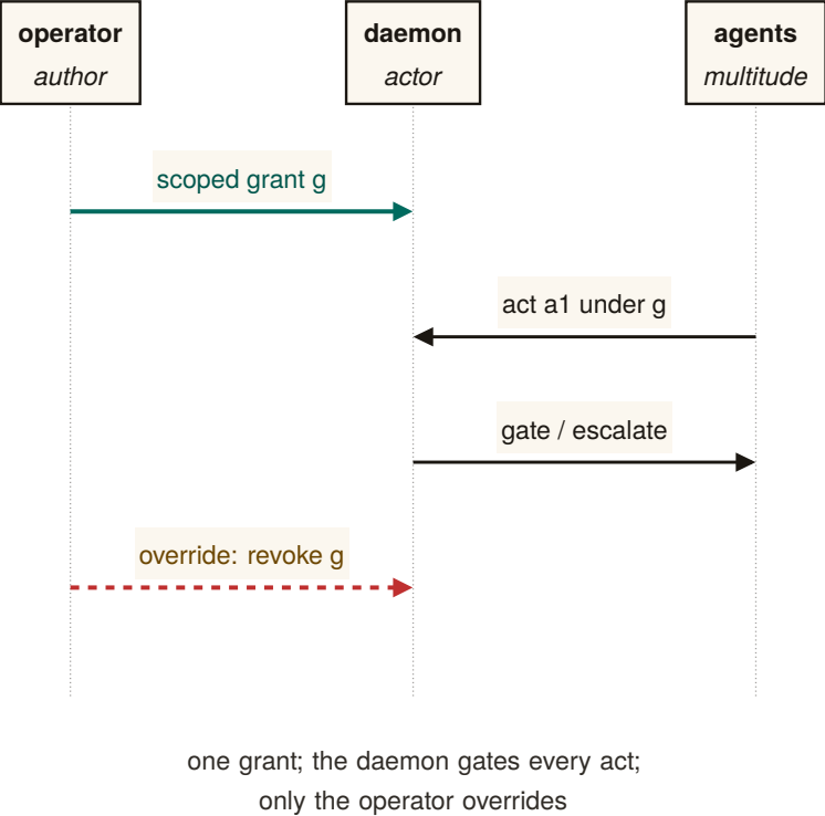
Figure 4.7: The grant-and-gate sequence, three lifelines and four messages, no crossing. The operator grants once (message 1: scoped grant g). Agents act under that grant (message 2), and the daemon gates or escalates every such act (message 3) rather than granting again. The override (message 4) is the one edge running straight from operator to daemon, bypassing the agents entirely. Idealized to one representative act; a live fleet repeats messages 2–3 per act, not per grant [internal].
