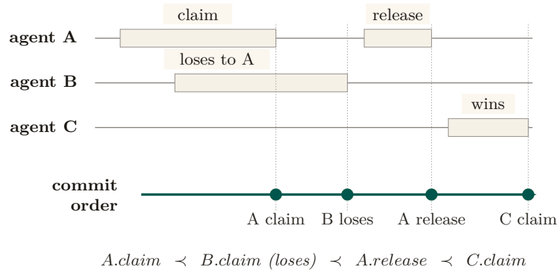
Figure 11: A real-time history and its extracted linearization. Operations overlap in caller time, but each receives one commit point on the single writer’s rail, and the linearization reads: A claims, B loses, A releases, C claims. The claim is conditional on one writer, no uncommitted reads, and replies after commit. [internal]
