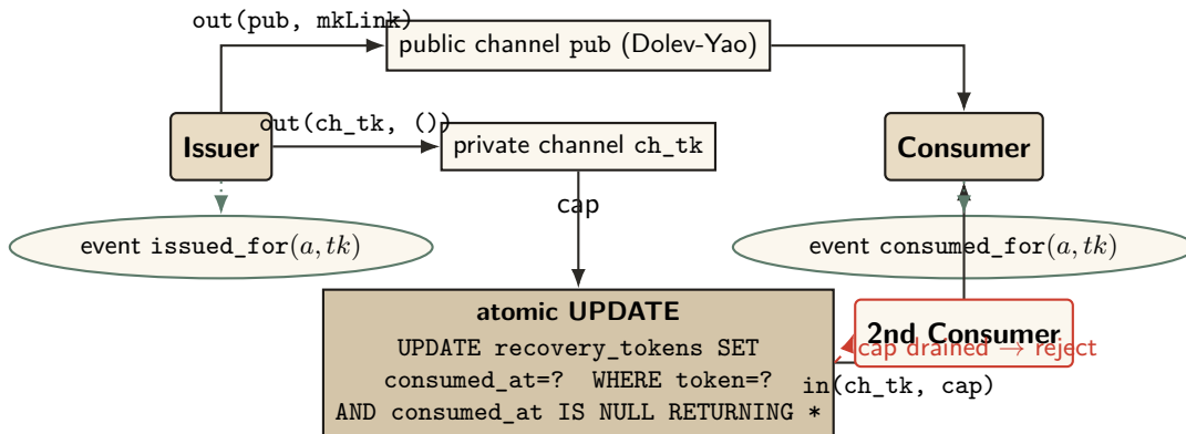
Figure 6: Magic-link single-use atomicity. The SQL UPDATE ...WHERE consumed_at IS NULL RETURNING is the runtime analogue of the ProVerif private-channel cap : SQLite serializes concurrent writers, so the first caller drains the cap and the second consumer’s transaction returns zero rows. Verified properties: injective single-use ( \text{inj-event}(\text{consumed\_for}) \Rightarrow \text{inj-event}(\text{issued\_for}) ) and binding.
