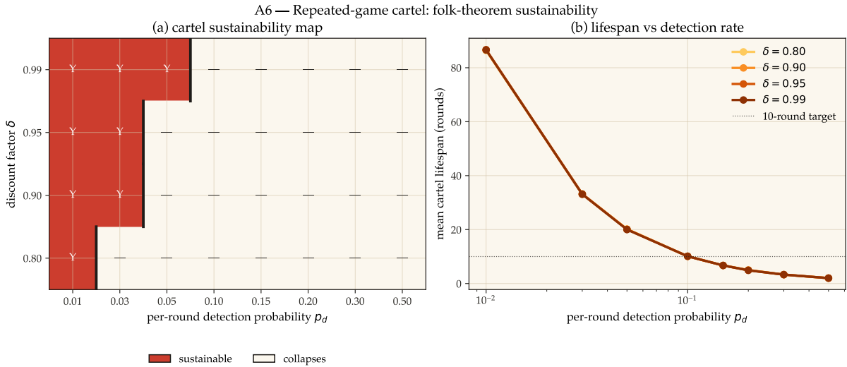
Figure 10: A6 — Repeated-game cartel folk-theorem. Left: sustainability map over the (p_d, \delta) grid; red cells are configurations where the grim-trigger cartel beats one-shot defection in expected PV (sustainable), white cells are where it does not (collapses). The thick black vertical bars mark the per-row threshold p_d^* . Right: mean cartel lifespan (rounds until first detection) vs. p_d , one line per discount factor \delta . At the realistic \delta = 0.95 , p_d^* \approx 0.10 : protocols must achieve \geq 10\% per-round detection to break repeated-game cartels.
