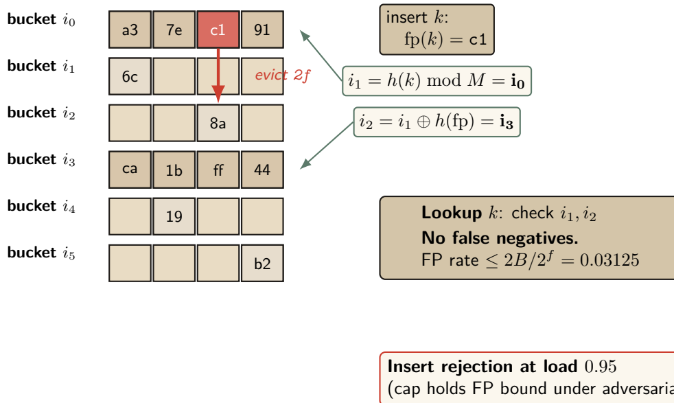
Figure 8: Cuckoo filter (Fan et al. [23]). 8-bit fingerprints, 4 entries per bucket, partial-key cuckoo hashing. Insert lands at either of two candidate buckets i_1, i_2 = i_1 \oplus h(\text{fp}) ; on full, evict and re-insert at the kicked fingerprint's alternate. The runtime caps load factor at 0.95 to keep occupancy inside the regime where the false-positive bound holds.
