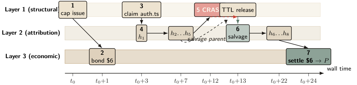
Figure 11: Worked-example timeline (App D). Three swimlanes for the three architectural layers; events placed by wall-clock minute on the x -axis. Layer 1 (structural) issues the capability at t_0 , releases on TTL after crash, and re-issues for the successor. Layer 3 (economic) posts $6 in escrow at t_0 + 1 and settles at t_0 + 24 . Layer 2 (attribution) accumulates evidence-chain entries h_1 – h_5 on \alpha ’s timeline and h_6 – h_8 on \beta ’s, linked by an explicit salvage parent edge so attribution survives the identity disposal at minute 12.
