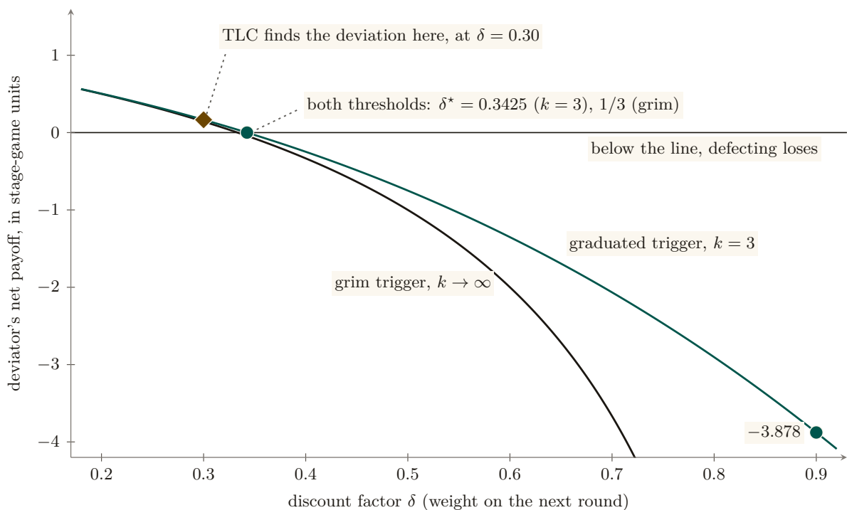
Figure 3: Net payoff to a player who defects once, against the discount factor, under the two punishment regimes of this section. The two curves cross zero 0.0092 apart — \delta^* = 0.3425 for the three-round graduated trigger, 1/3 for grim trigger — so bounding the punishment at three rounds costs almost nothing in the threshold. Away from the threshold the two regimes are not close at all: grim trigger’s punishment grows without bound and leaves the frame at \delta = 0.722 , where it reaches the axis floor, while the graduated trigger’s stays finite, reaching the chapter’s worked value of -3.878 at \delta = 0.9 . The marked point at \delta = 0.30 is the one discount factor whose model-checker transcript is committed — the session printed below — and its height, 0.166, is that run’s own closing margin, so the sign there, defecting still pays, is what the run reports. Both curves are the section’s own closed form at (c, d, p) = (3, 4, 1) , not a simulation [verified, proofs/economics/delta-threshold.z3 and claim_signaling_delta30.run.log ].
