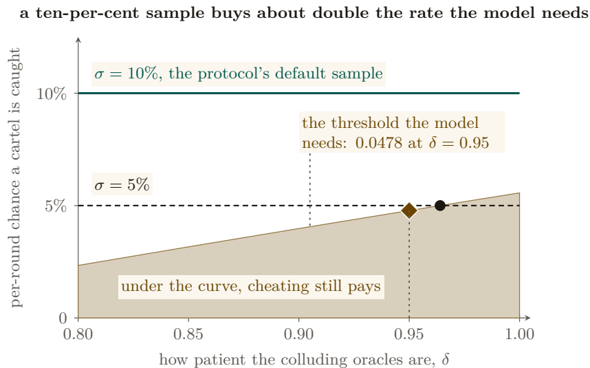
Figure 4: The default human-audit sample is roughly twice the detection rate the cartel model demands, and a halved sample is not. The amber curve is the chapter’s own fragility threshold, the per-round detection probability at which a colluding oracle pair stops preferring the cartel, drawn from (\pi_C - (1 - \delta)\pi_D)/(L + \delta\pi_D) at the supplied payoffs \pi_C = 5/3 , \pi_D = 4.95 , L = 25 ; below it collusion still pays. Because the human-audit sampling rate is the oracle layer’s detection probability, the protocol’s default \sigma = 10\% is the flat teal rule, and it clears the threshold at every patience the model admits – 0.0478 at \delta = 0.95 , and never more than 0.0557 even as \delta \rightarrow 1 . A 5% sample clears it only until \delta = 0.964 ; past that the cheaper sample silently licenses exactly the 2-of-3 oracle collusion the audit exists to price. The threshold is model-conditional: a different payoff spread, event timing, or monitoring model moves the whole curve, and the deployed detector is not claimed to attain it. [verified; figures/data/oracle-audit-threshold.csv from figures/data/make-figure-data.py, deterministic]
