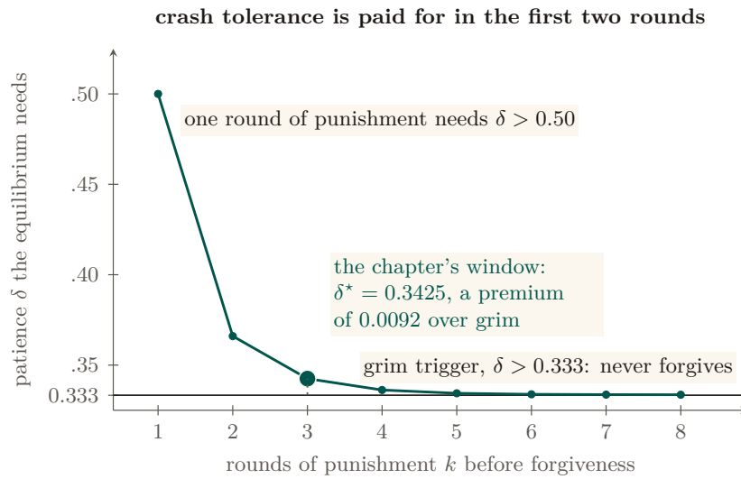
Figure 2: A forgiving punishment window is almost free, and the whole price is paid in the first two rounds. The smallest patience at which truthful file-claim signalling survives a k -round graduated trigger, at the chapter's stage game ( d - c = 1 , c - p = 2 ), against the grim-trigger floor \delta > 1/3 that a never-forgiving strategy needs. One round of punishment demands \delta > 0.500 ; two rounds already fall to 0.366; the three-round window the chapter adopts costs 0.3425, a premium of 0.0092 over grim, and by five rounds the premium falls under 0.001. This is why the production strategy can afford to forgive: crashes and deliberate defection are indistinguishable to an observer, and buying that tolerance costs almost no patience. The curve is the root of 2(\delta + \dots + \delta^k) = 1 and holds only for this stage game; a different payoff spread moves every point. [verified; figures/data/graduated-trigger-threshold.csv from figures/data/make-figure-data.py, deterministic]
