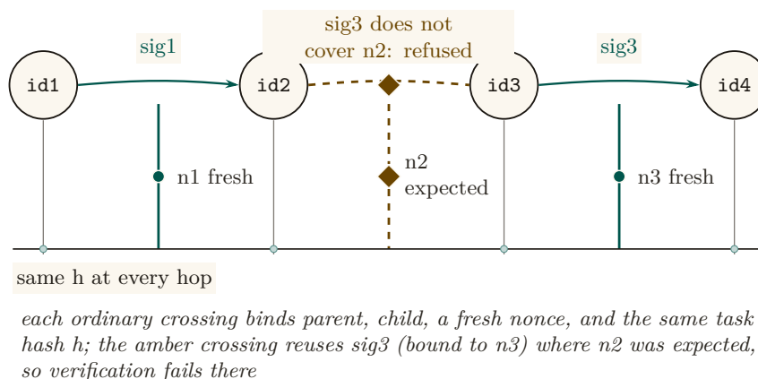
Figure 4: The delegation chain as a signed provenance braid across four identities id1–id4. Ordinary hops 1 and 3 bind parent, child, a fresh nonce (n1, n3), and the shared task hash h below. Hop 2 shows a splice attack: an attacker moves the legitimate signature sig3 (computed over id3, id4, and n3) into the id2–id3 position, where the verifier expects a signature over n2; the check fails at exactly that crossing, so the discontinuity is visible at one adjacent-identity boundary rather than anywhere else in the chain. [internal]
