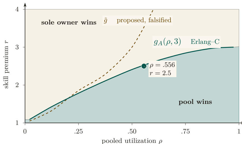
Figure 3: The specialization boundary at a three-agent pool. Below the Erlang-C boundary g_A(\rho, 3) (teal), pooling wins; above it, sole ownership wins — the two regions are now filled and edged, not hatched. The superseded threshold \tilde{g} (dashed) is kept for comparison: it diverges rather than saturating at the pool capacity ratio. The worked instance ( \rho = .556 , r = 2.5 ) narrowly clears the correct boundary into the sole-owner region [internal, closed form].
