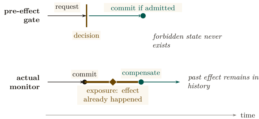
Figure 6: The reference-monitor test as a causal counterfactual. A true mediator decides before the commit point, so a forbidden state never exists. The present policy monitor instead subscribes after commit: the caution segment is the exposure interval in which the effect has already happened, before it can observe, halt subsequent work, and compensate. Only uniqueness constraints and fail-closed boot gates belong to the upper trace; subscriber rules belong to the lower one. [internal]
