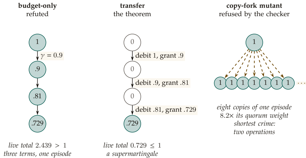
Figure 5.3: Three lineages of one witnessed episode of weight 1, derived at \gamma = 0.9 . Under the budget-only phrasing every derivation stays live and the closure sums to 0.9+0.81+0.729 = 2.439 > 1 : reputation minted from nothing, which is why that phrasing was refuted before proving. Under transfer each derivation grants the child \gamma w_p and debits the source w_p , so only the leaf is live and the total never exceeds what was witnessed. The copy-full mutant, which forks the undebited record, turns one episode into 8.2 \times its quorum weight in two operations, and the checker refuses it. [verified for the chain by hand; internal, a6_no_mint.py, seed 20260816]
