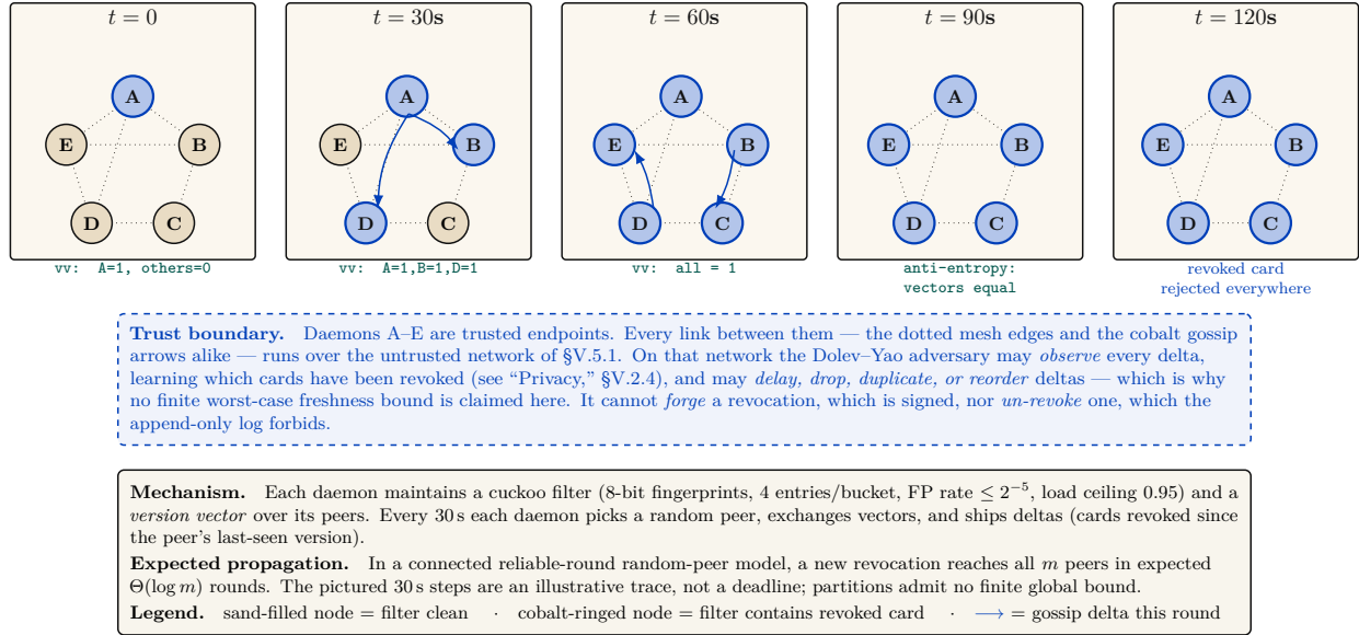
Figure V.6: A single revocation reaches every daemon in the mesh through anti-entropy gossip alone, in expected \Theta(\log m) rounds under the stated connected reliable-round model, with no worst-case time guarantee under partition. At t = 0 daemon A locally revokes a Harbor Card (its filter and revocation table); gossip then ships deltas to random peers every 30 s. The panels show one possible execution, not a deadline. Version vectors make duplicate and reordered deltas idempotent once delivered, but do not heal an unbounded partition. The dashed strip beneath the panels states the trust boundary the panels themselves cannot draw: the daemons are trusted, every wire between them is not.
