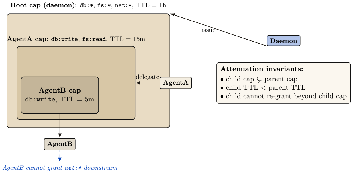
Figure V.2: Every delegated capability is a strict subset of its parent’s, in both rights and TTL, so a chain of delegations can only narrow authority, never widen it. AgentB inherits only what AgentA explicitly delegates and cannot re-grant capabilities it does not hold. This is enforced both at issuance (the parent signs over the child’s attenuated claim set) and at verification (the verifier checks the chain of is_subset relations).
