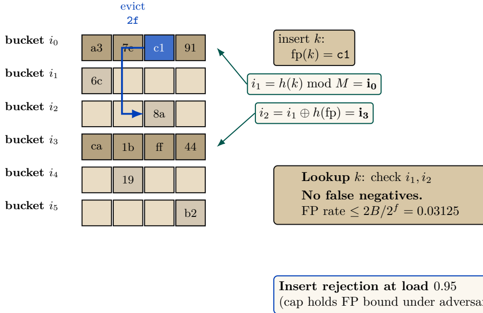
Figure V.5: Cuckoo-filter revocation gate (Fan et al. [37]) with the load-factor ceiling that defeats the pollution attack. Insert lands at either of two candidate buckets i_1, i_2 = i_1 \oplus h(fp) ; on full, evict and re-insert at the kicked fingerprint’s alternate. Insert rejection at 0.95 caps occupancy inside the regime where the false-positive bound holds.
