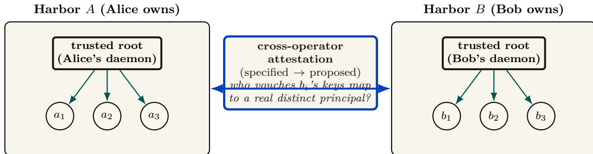
Figure IV.4: The market rests on a keystone it does not yet have: local non-forgeable identity covers only a single trusted daemon, while the market is defined by operators who share no such root. Chapters I–III rest on local non-forgeable identity : a per-agent identity no agent can edit within one trusted daemon — a single trusted root that vouches for every agent it mints. That is exactly what a single-operator harbor needs. But the market is defined by mutually-distrusting operators trading across a boundary neither controls, and that primitive explicitly disclaims the relevant threat model (intra-fleet, not a cross-party PKI, no hostile-operator defense). Binding signing keys across harbors you do not own is a different, unsolved problem: cross-operator attestation . Across the boundary, the counterparty’s daemon is the adversary the local threat model declares out of scope, and the witness log gives log integrity , not identity binding . It is the highest-leverage unbuilt keystone, and it gates the entire market thesis.
