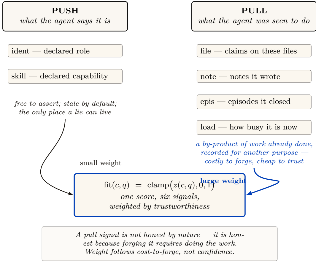
Figure I.10: The discovery ranker weights pull signals — residue of work a candidate actually did, recorded for some other purpose — over push signals, what a candidate merely declares about itself (Eq. I.4, Table I.5). The design weights pull over push not because declarations are usually false but because they are free — an agent that wants to be routed work can inflate a skill tag at no cost and cannot inflate a merged episode without merging something. This is the discovery-side instance of the same discipline digest-with-zoom (Def. I.3.1) applies to summaries: trust the claim that reaches an artifact.
