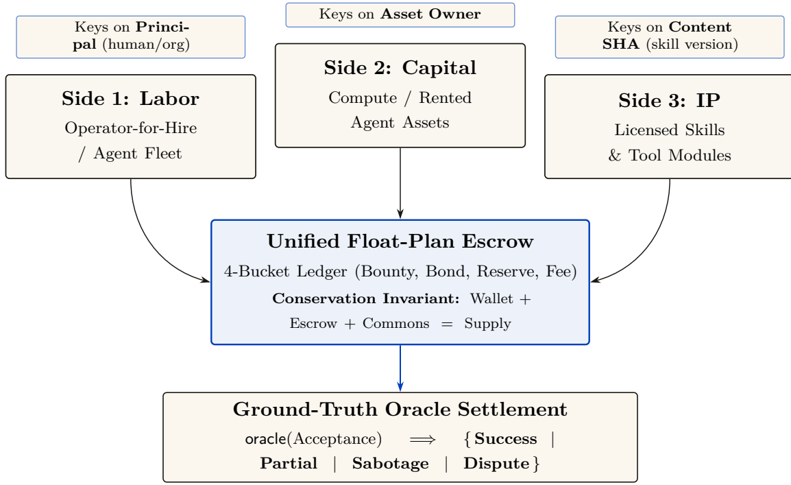
Figure IV.2: Labor, capital, and IP are three distinct incentive constraints — not three UI tabs — that settle on one escrow but key reputation on three different identity objects. Labor, capital (rented agents), and IP (licensed skills) all settle on a single float-plan escrow, so conservation holds globally without a second ledger. This is the categorical heart of the design: the three sides are isomorphic at the conservation object (the escrow) and non-isomorphic at the identity object (each side keys reputation on a different entity, the dashed band). Calling it “one structure, three decorations” without that qualifier is a decorative-analogy failure. The rider is mandatory: the market is three-sided by design and two-sided in shipped reality, because sides 2 and 3 presuppose a non-forgeable, durable identity (§IV.6). The economics per side: labor’s margin is bounty – slashed sub-bonds – fee; capital’s renter holds the runtime jail while the owner bears reputation; IP is metered with clawback, paid only on green settlement. The escrow and its conservation invariant are implemented and property-tested.
