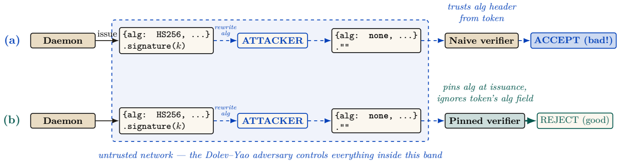
Figure V.3: Pinning the verification algorithm at issuance — rather than trusting the token’s self-declared alg field — closes the algorithm-confusion attack that a naive verifier admits. The dashed band is the chapter’s trust boundary: the daemon and the verifier sit outside it, and everything inside it is under the control of the Dolev–Yao adversary of §V.5.1, who may read, rewrite, or inject any token in flight. (a) A naive verifier trusts the alg field of the incoming token; an attacker inside the band rewrites alg=HS256 to alg=none , strips the signature, and the verifier accepts an unauthenticated message. (b) The pinned verifier records the issuance algorithm out-of-band — across the boundary, where the adversary cannot reach — then re-checks each token against the pinned algorithm rather than the token’s self-described one. The ProVerif model encodes both verifiers and shows the naive path produces a counter-trace witness for the rewrite, while the pinned path admits no such trace. Runtime conformance: 5 attack patterns + 2 controls, all pass.
