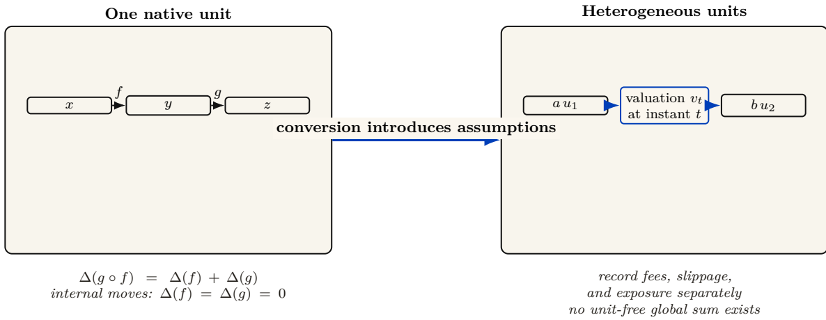
Figure IV.5: Conservation composes exactly within one unit of account but not across currencies without further assumptions. In one native unit, the supply delta of a composed trace is the sum of its step deltas, so zero-delta internal operations remain conservative. A cross-currency transfer is different: it requires a named valuation function and instant, plus explicit fee, slippage, and exposure accounts. Category-theoretic language does not remove those accounting assumptions.
