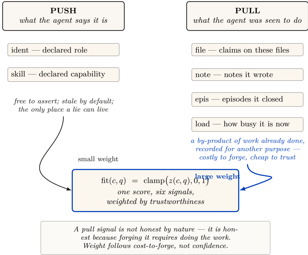
Figure 10: The discovery ranker weights pull signals — residue of work a candidate actually did, recorded for some other purpose — over push signals, what a candidate merely declares about itself (Eq. 4, Table 5). The design weights pull over push not because declarations are usually false but because they are free — an agent that wants to be routed work can inflate a skill tag at no cost and cannot inflate a merged episode without merging something. This is the discovery-side instance of the same discipline digest-with-zoom (Def. 3.1) applies to summaries: trust the claim that reaches an artifact.
