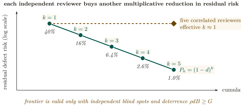
Figure 10: Purchased assurance is one risk-cost trajectory. Each teal point adds one independently bonded reviewer: cumulative cost rises linearly while residual defect risk falls geometrically. At d = .6 , three reviewers leave 6.4% residual risk and five leave about 1%. The dashed amber counterfactual charges for five correlated reviewers but delivers roughly one reviewer’s protection. Independence and Becker deterrence \rho dB \geq G are therefore conditions of the frontier, not footnotes to headcount.
