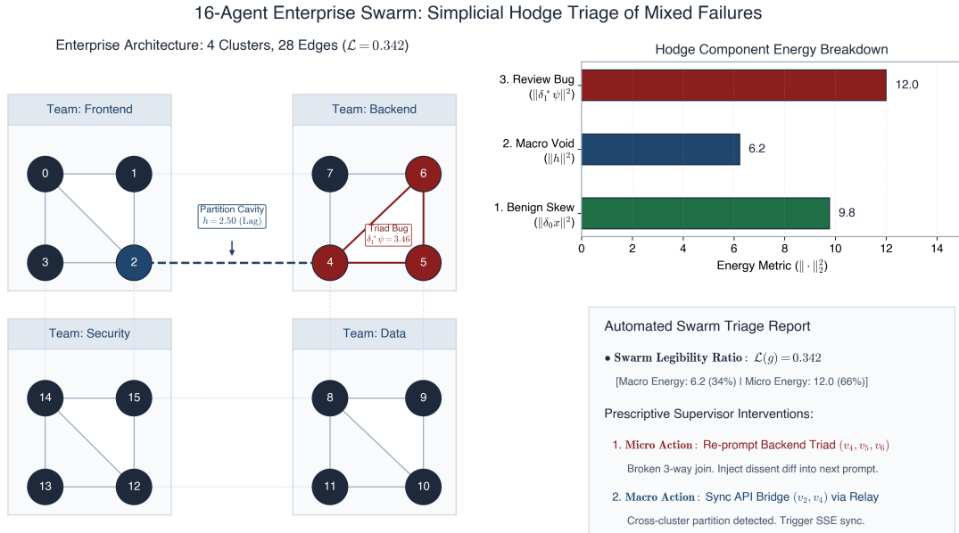
Figure 6: 16-agent enterprise swarm triage under mixed failure. The Backend Team experiences an internal review hallucination ( \delta_1^* \psi = 3.46 ), while cross-team bridge ( v_2, v_4 ) experiences an uninspected network partition lag ( h = 2.50 ). The Swarm Legibility Ratio \mathcal{L}(g) = 0.342 decomposes the failure into 65.8% micro-triad bug and 34.2% macro-partition cavity.
