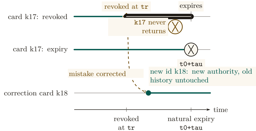
Figure 6: Acceptance is a one-way interval attached to one card ID. Card k17 stops being admissible either at explicit revocation (tick \mathbf{tr} ) or at natural expiry (tick \mathbf{t0+tau} ) and never re-enters the valid set. If revocation was a mistake, the operator issues k18 on a new lane: new authority on a new ID, with the rejected history on k17 left untouched rather than mutated. [internal]
