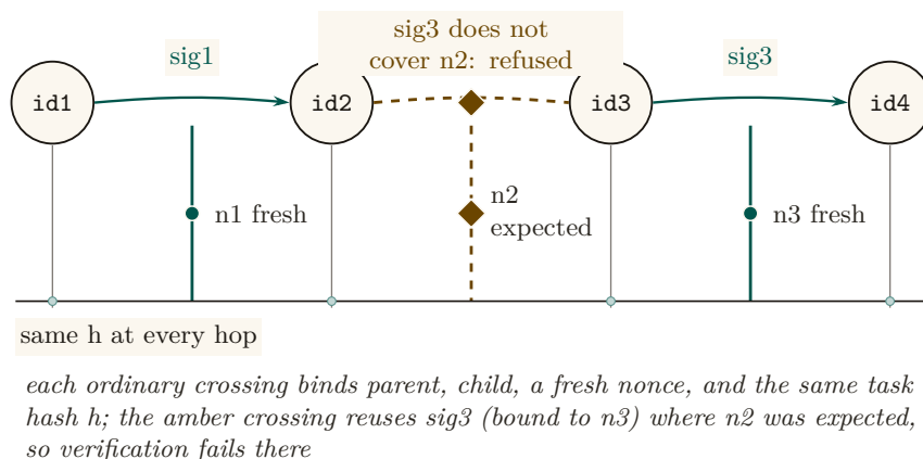
Figure 3: The delegation chain as a signed provenance braid across four identities id1–id4. Ordinary hops 1 and 3 bind parent, child, a fresh nonce ( n1 , n3 ), and the shared task hash h ; the amber crossing reuses sig3 (computed over id3, id4, and n3 ) into the id2–id3 position, where the verifier expects a signature over n2 ; the check fails at exactly that crossing, so the discontinuity is visible at one adjacent-identity boundary rather than anywhere else in the chain. [internal]
