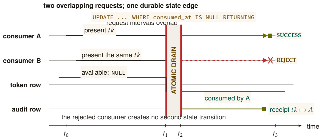
Figure 7.10: Single-use redemption is a concurrency property, not a two-arrow icon. Two consumers present the same account-bound token during one overlap window. Both requests reach the same serialized SQL update, but the token row has only one falling edge: the first transaction changes consumed_at from NULL and returns a row; the second observes the durable state and returns none. The audit rail records the winning consumer without creating another success path.
