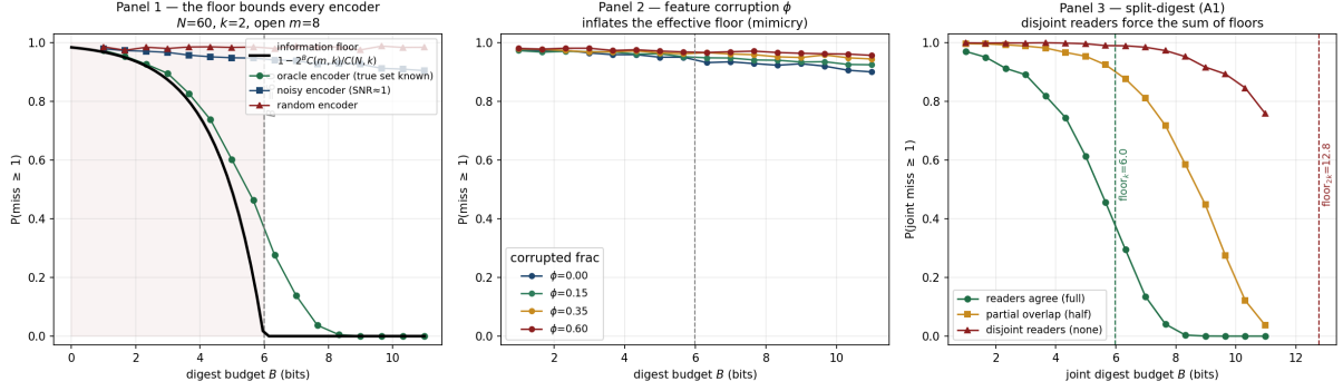
Figure 1: Panel 1: every encoder sits on or above the information floor (black); the oracle hugs it from above, the noisy and random encoders pay a premium — the floor bounds all of them, as predicted. Panel 2: corrupting a fraction \phi of features (the mimicry attack, Solution 6.5*) inflates the effective floor. Panel 3: two readers — when their load-bearing sets are disjoint (red), the joint miss curve shifts toward the 2k floor at 12.8 bits, versus the single-reader floor at 6.0; the visual confirmation of A1’s super-additive penalty.
