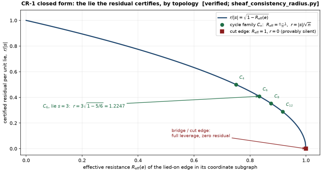
Figure 4: The CR-1 closed form: certified residual per unit lie, r/|s| = \sqrt{1 - R_{\text{eff}}(e)} , against the effective resistance of the lied-on edge in its coordinate subgraph. The cycle family C_n sits at R_{\text{eff}} = \frac{n-1}{n} (the harness’s C_6 point marked, 3\sqrt{1 - 5/6} = 1.2247 ); the cut-edge corner R_{\text{eff}} = 1 is provable silence [verified; closed form exact on C_4 – C_{12} and 200 random graphs, sheaf_consistency_radius.py ].
