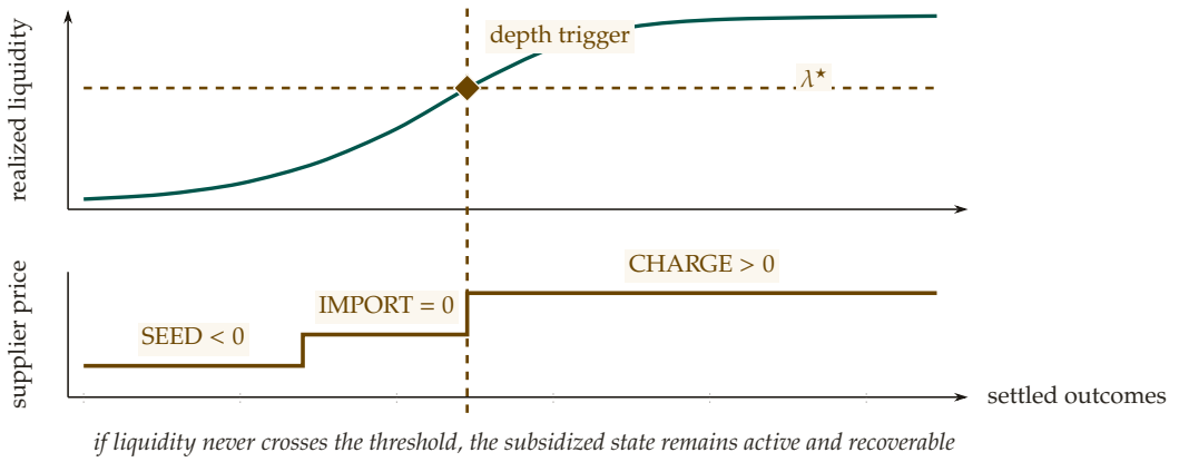
Figure 6.4: Cold start separates the measured market state from the policy schedule. The upper trace is realized liquidity over settled outcomes. The lower trace is the supplier-price regime applied to that state: seed supply below zero, credit imported work at zero, then charge only after liquidity crosses \lambda^* . The shared vertical trigger makes the dependency explicit. Calendar time is absent, and a market that never crosses the threshold does not silently advance to the charging regime.
