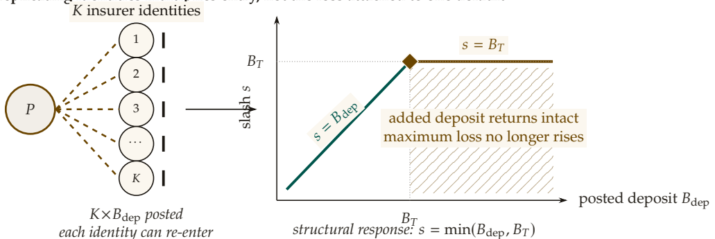
Figure 7.3: Deposit-only Sybil deterrence saturates. One principal can fund K interchangeable identities, but the loss attached to a defaulting identity rises only until its deposit reaches the transaction coverage B_T . Past that knee, s = \min(B_{\text{dep}}, B_T) = B_T : additional posted capital returns intact on no-loss transactions and cannot increase the attacker’s maximum loss. Figure 7.4 shows the corresponding simulated profit and commons-deficit sweeps.
