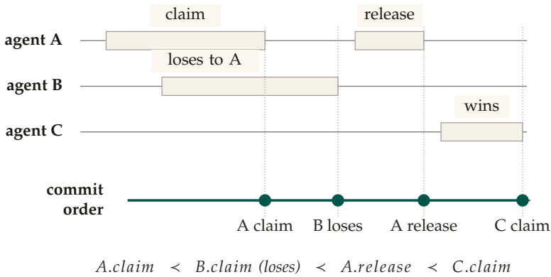
Figure 1.11: A real-time history and its extracted linearization. Operations overlap in caller time, but each receives one commit point on the single writer’s rail, and the linearization reads: A claims, B loses, A releases, C claims. The claim is conditional on one writer, no uncommitted reads, and replies after commit. [internal]
