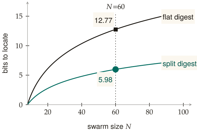
Figure 4.5: Bits an operator must read to locate the critical artifact, at the lower bound of Thm. 4.6.1 with m=8 , k=2 . One flat digest serving both readers jointly needs \text{Floor}(N, 4, 8) bits; two split digests, one per reader, each need only \text{Floor}(N, 2, 8) . At N=60 the split digest costs 5.98 bits against the flat digest's 12.77 — a 2.13\times penalty, not the 2\times that halving the readers would predict. The committed sweep CSV ( r1-floor.csv ) is not yet present, so the two curves are the chapter's own closed-form \text{Floor} formula rather than simulated points; only the N=60 values it works by hand are marked [internal].
