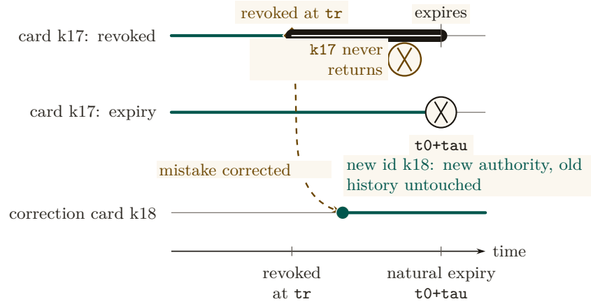
Figure 6: Acceptance is a one-way interval attached to one card ID. Card k17 stops being admissible either at explicit revocation (tick tr ) or at natural expiry (tick t_0+\tau ) and never re-enters the valid set. If revocation was a mistake, the operator issues k18 on a new lane: new authority on a new ID, with the rejected history on k17 left untouched rather than mutated. [internal]
